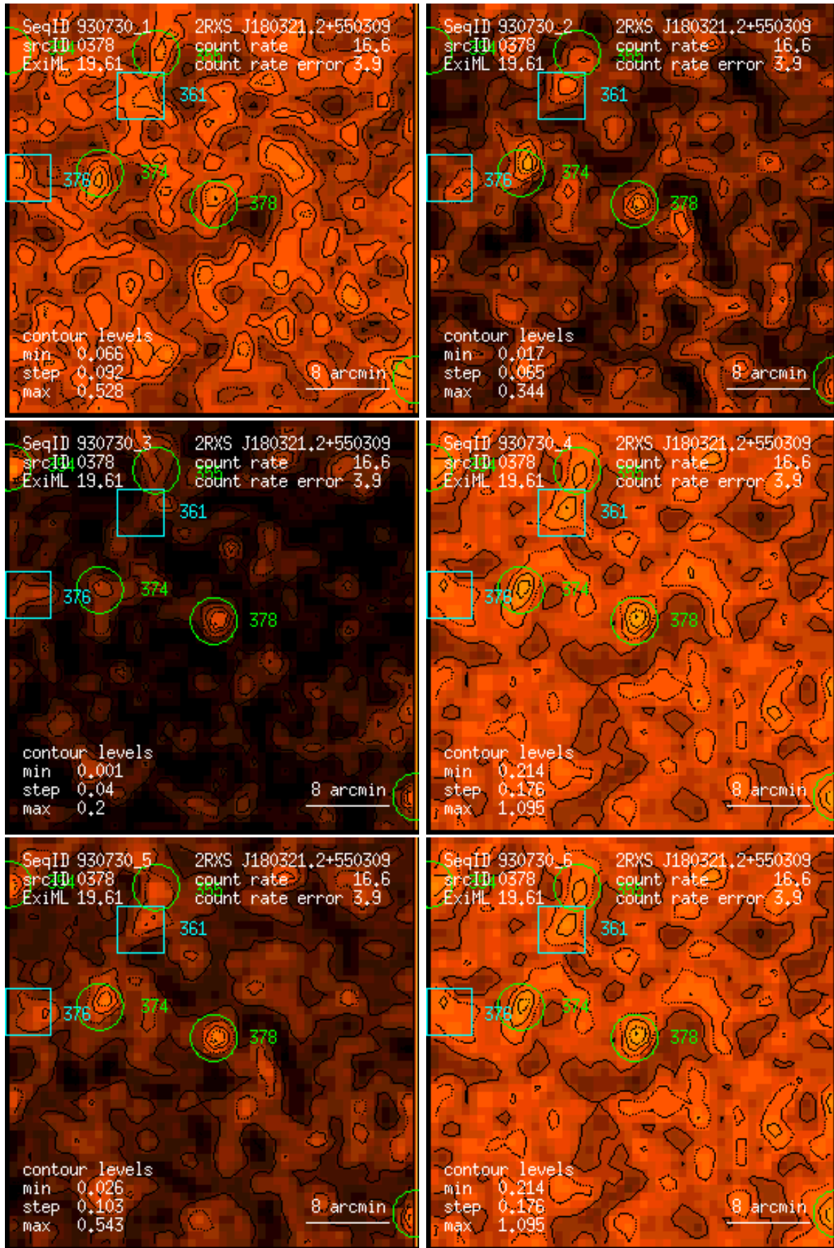
Figure 378: RASS 930730: detection 0378: band rate images, Gaussian filter: (1) PSPC channels 11 – 41, (2) 52 – 90, (3) 91 – 201, (4) 11 – 235, (5) 52 – 201, (6) 11 – 201. Broad band rates in counts/ks. Band rate contour levels in counts/ks/arcmin 2 .
