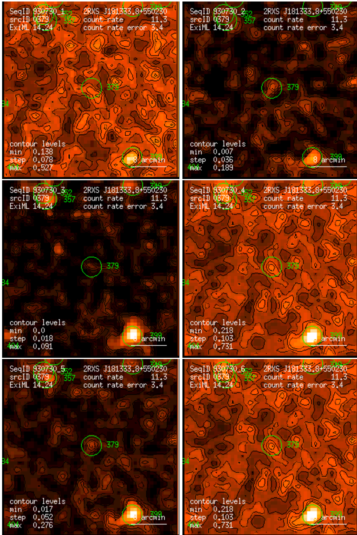
Figure 379: RASS 930730: detection 0379: band rate images, Gaussian filter: (1) PSPC channels 11 – 41, (2) 52 – 90, (3) 91 – 201, (4) 11 – 235, (5) 52 – 201, (6) 11 – 201. Broad band rates in counts/ks. Band rate contour levels in counts/ks/arcmin 2 .
