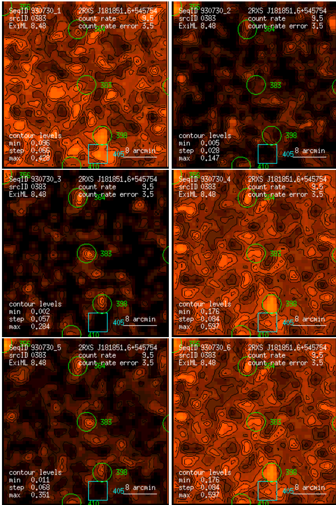
Figure 383: RASS 930730: detection 0383: band rate images, Gaussian filter: (1) PSPC channels 11 – 41, (2) 52 – 90, (3) 91 – 201, (4) 11 – 235, (5) 52 – 201, (6) 11 – 201. Broad band rates in counts/ks. Band rate contour levels in counts/ks/arcmin 2 .
