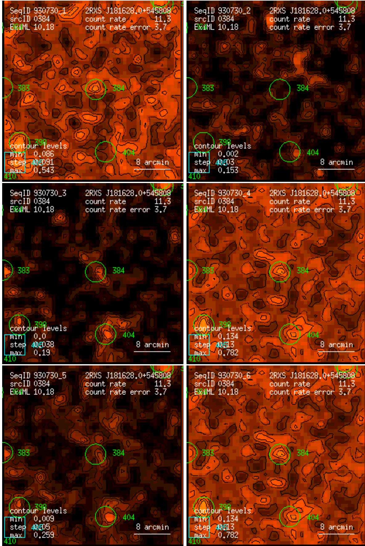
Figure 384: RASS 930730: detection 0384: band rate images, Gaussian filter: (1) PSPC channels 11 – 41, (2) 52 – 90, (3) 91 – 201, (4) 11 – 235, (5) 52 – 201, (6) 11 – 201. Broad band rates in counts/ks. Band rate contour levels in counts/ks/arcmin 2 .
