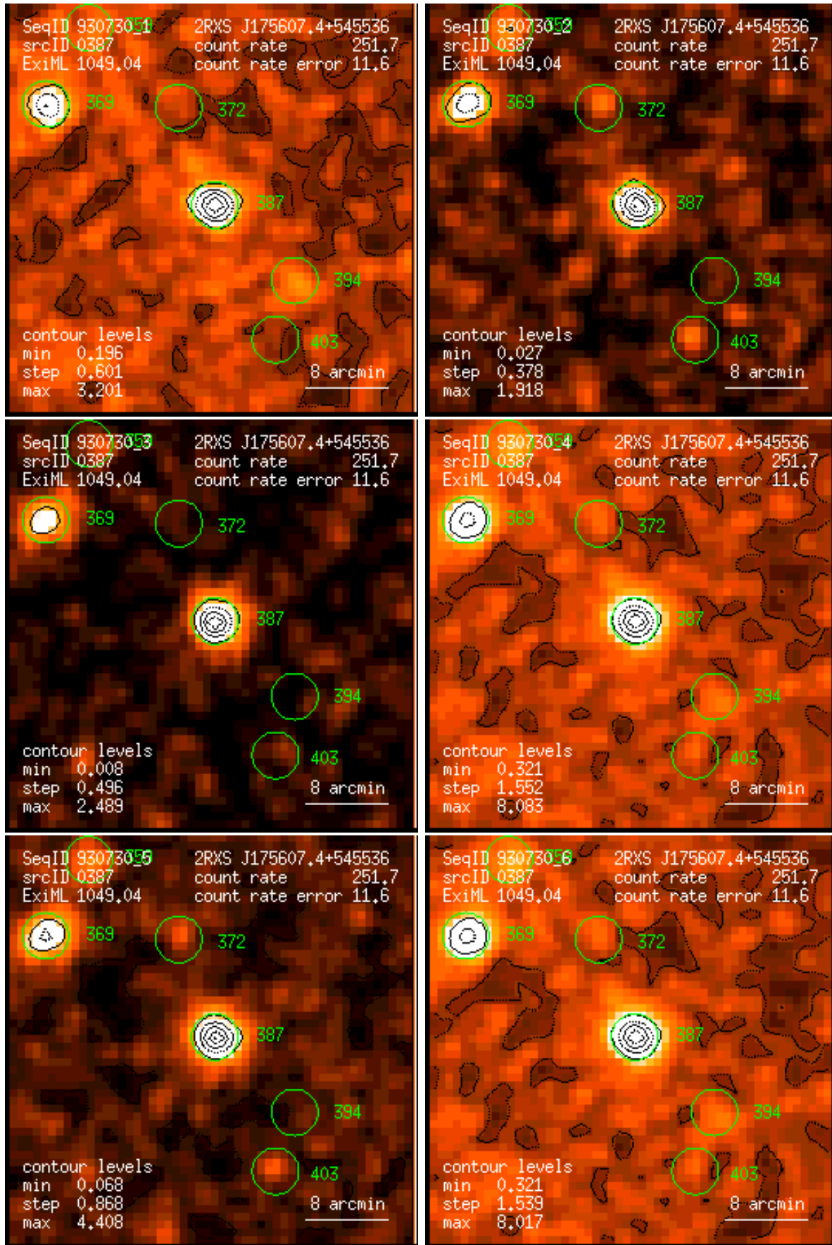
Figure 387: RASS 930730: detection 0387: band rate images, Gaussian filter: (1) PSPC channels 11 – 41, (2) 52 – 90, (3) 91 – 201, (4) 11 – 235, (5) 52 – 201, (6) 11 – 201. Broad band rates in counts/ks. Band rate contour levels in counts/ks/arcmin 2 .
