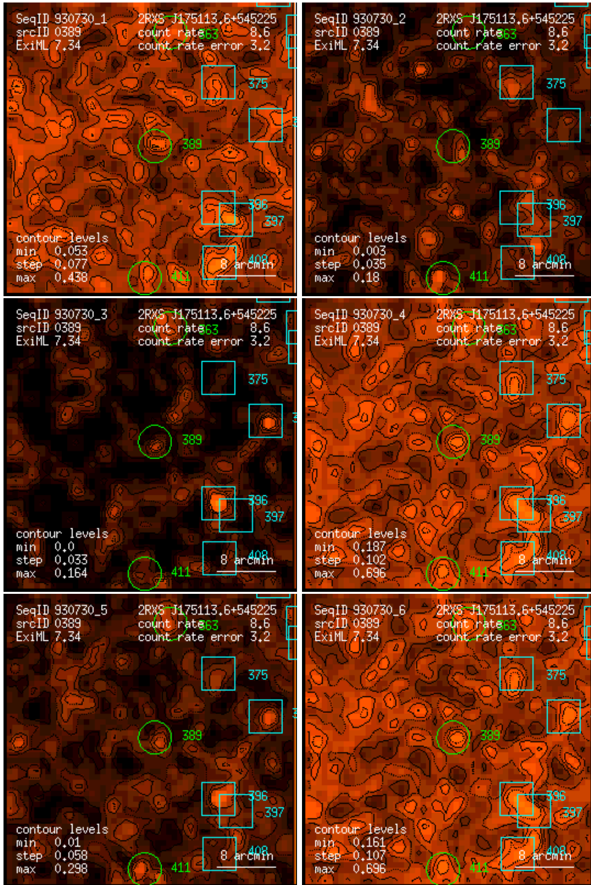
Figure 389: RASS 930730: detection 0389: band rate images, Gaussian filter: (1) PSPC channels 11 – 41, (2) 52 – 90, (3) 91 – 201, (4) 11 – 235, (5) 52 – 201, (6) 11 – 201. Broad band rates in counts/ks. Band rate contour levels in counts/ks/arcmin 2 .
