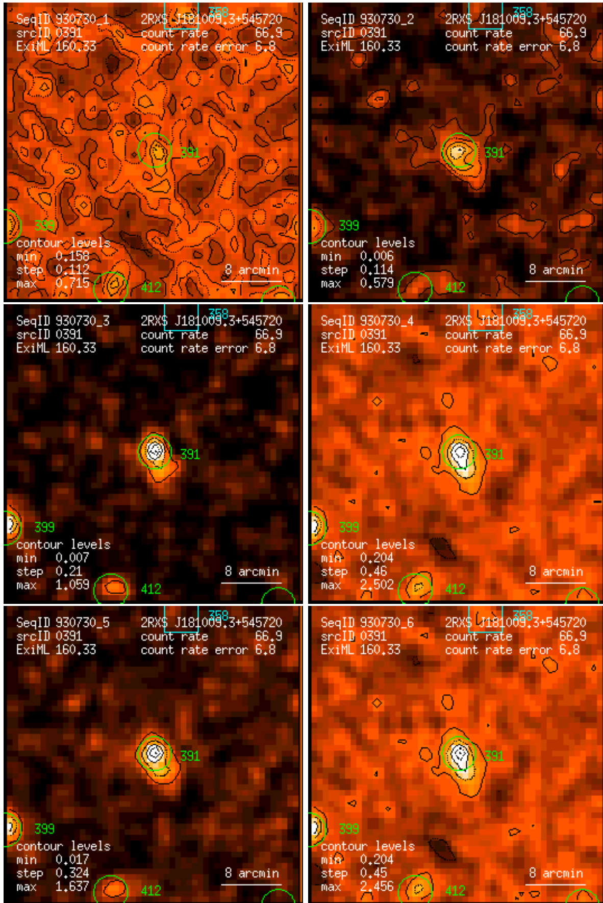
Figure 391: RASS 930730: detection 0391: band rate images, Gaussian filter: (1) PSPC channels 11 – 41, (2) 52 – 90, (3) 91 – 201, (4) 11 – 235, (5) 52 – 201, (6) 11 – 201. Broad band rates in counts/ks. Band rate contour levels in counts/ks/arcmin 2 .
