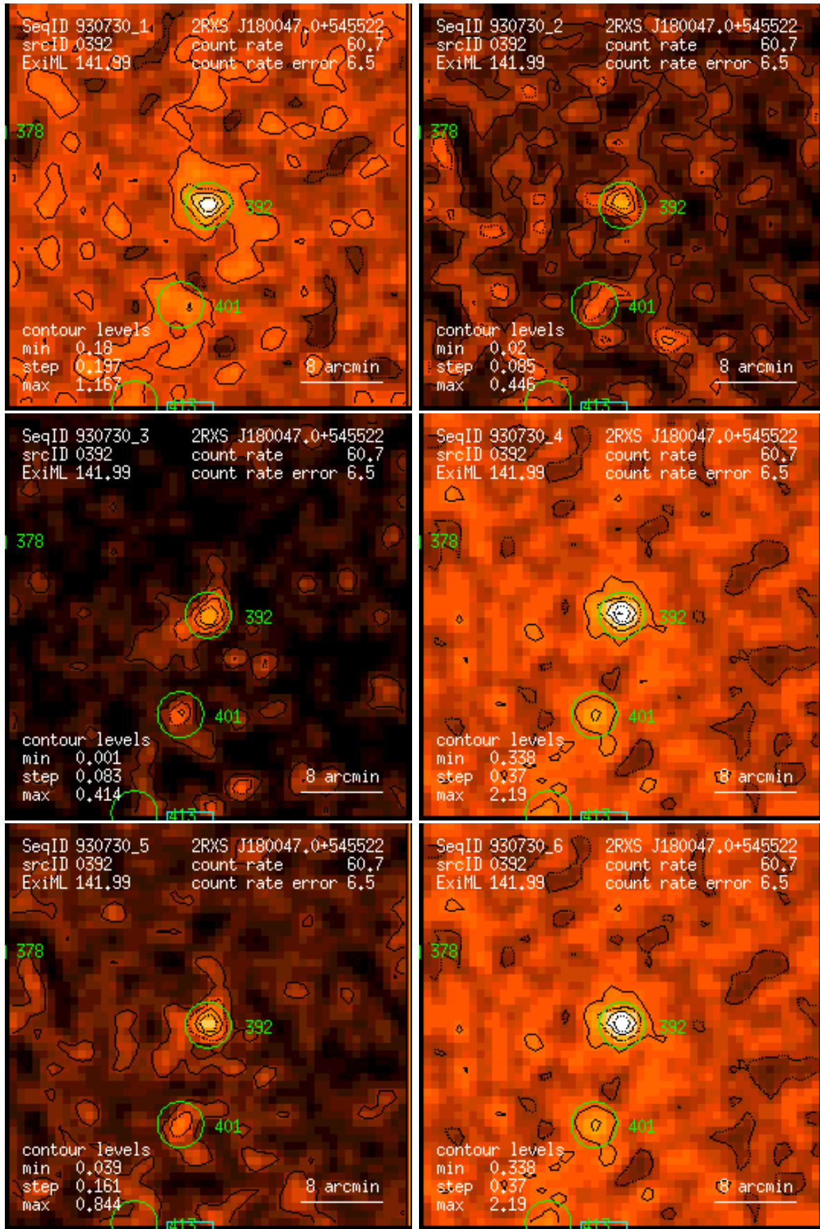
Figure 392: RASS 930730: detection 0392: band rate images, Gaussian filter: (1) PSPC channels 11 – 41, (2) 52 – 90, (3) 91 – 201, (4) 11 – 235, (5) 52 – 201, (6) 11 – 201. Broad band rates in counts/ks. Band rate contour levels in counts/ks/arcmin 2 .
