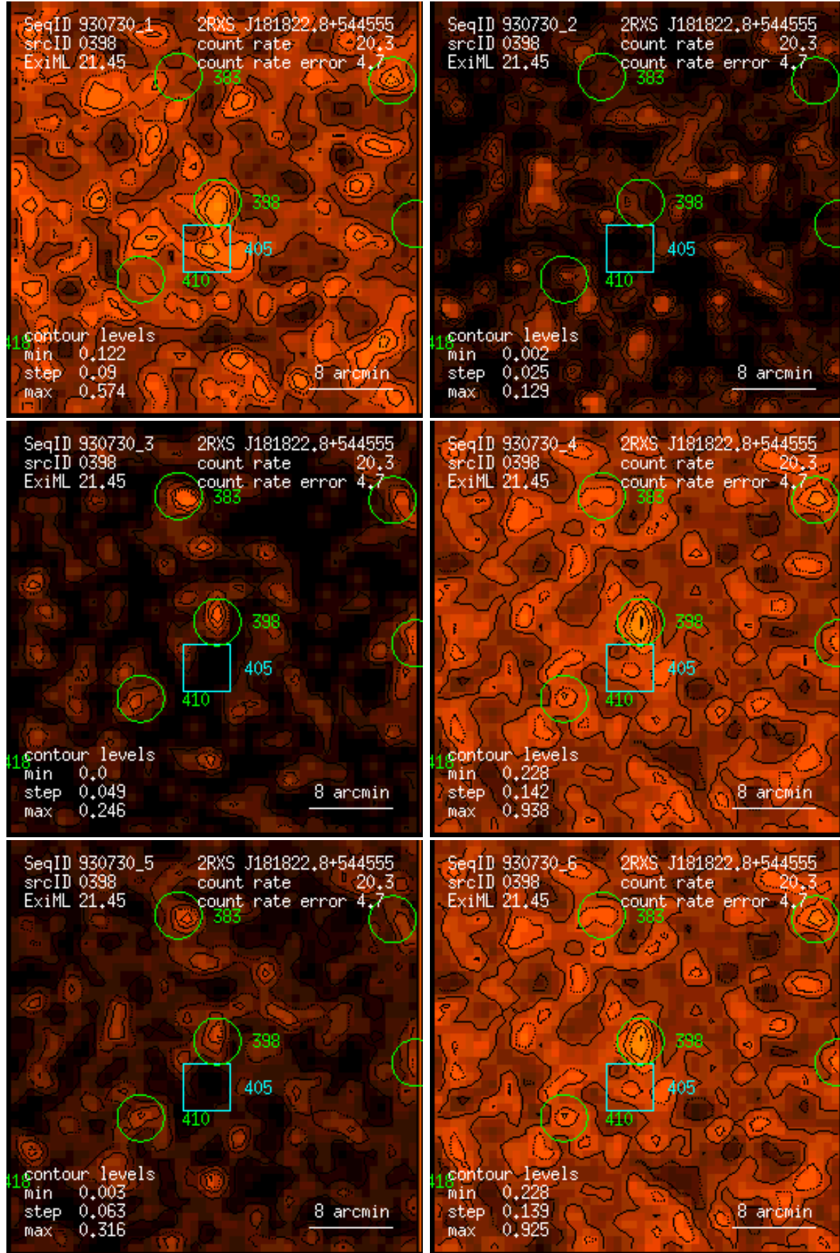
Figure 398: RASS 930730: detection 0398: band rate images, Gaussian filter: (1) PSPC channels 11 – 41, (2) 52 – 90, (3) 91 – 201, (4) 11 – 235, (5) 52 – 201, (6) 11 – 201. Broad band rates in counts/ks. Band rate contour levels in counts/ks/arcmin 2 .
