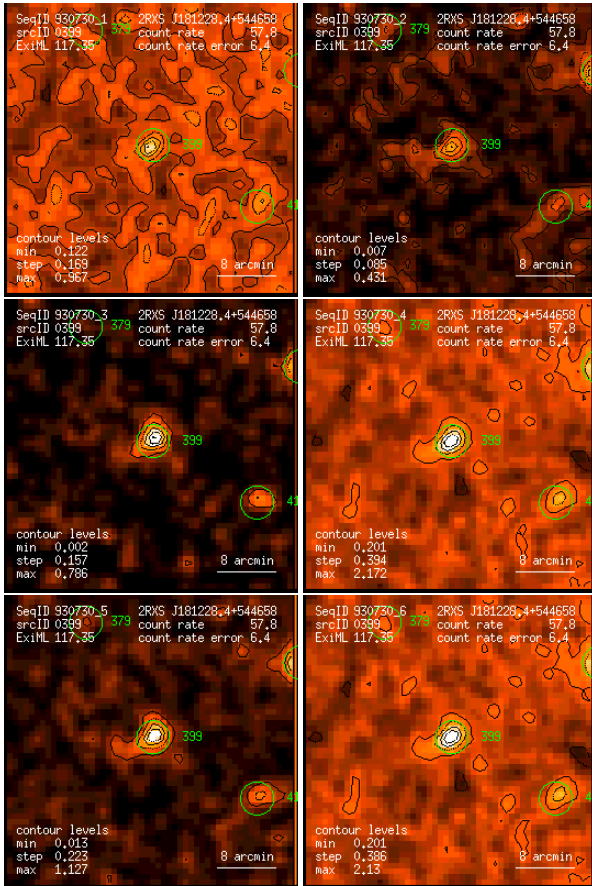
Figure 399: RASS 930730: detection 0399: band rate images, Gaussian filter: (1) PSPC channels 11 – 41, (2) 52 – 90, (3) 91 – 201, (4) 11 – 235, (5) 52 – 201, (6) 11 – 201. Broad band rates in counts/ks. Band rate contour levels in counts/ks/arcmin 2 .
