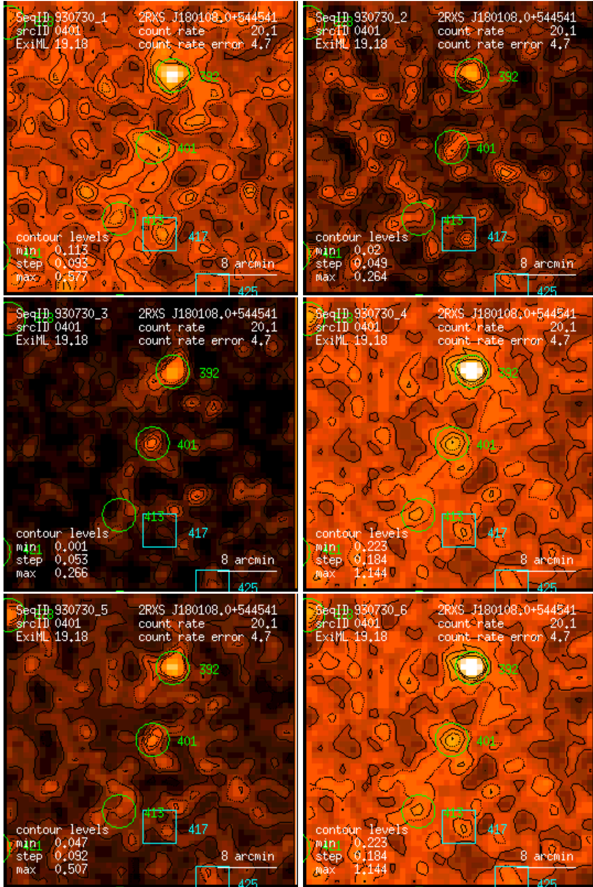
Figure 401: RASS 930730: detection 0401: band rate images, Gaussian filter: (1) PSPC channels 11 – 41, (2) 52 – 90, (3) 91 – 201, (4) 11 – 235, (5) 52 – 201, (6) 11 – 201. Broad band rates in counts/ks. Band rate contour levels in counts/ks/arcmin 2 .
