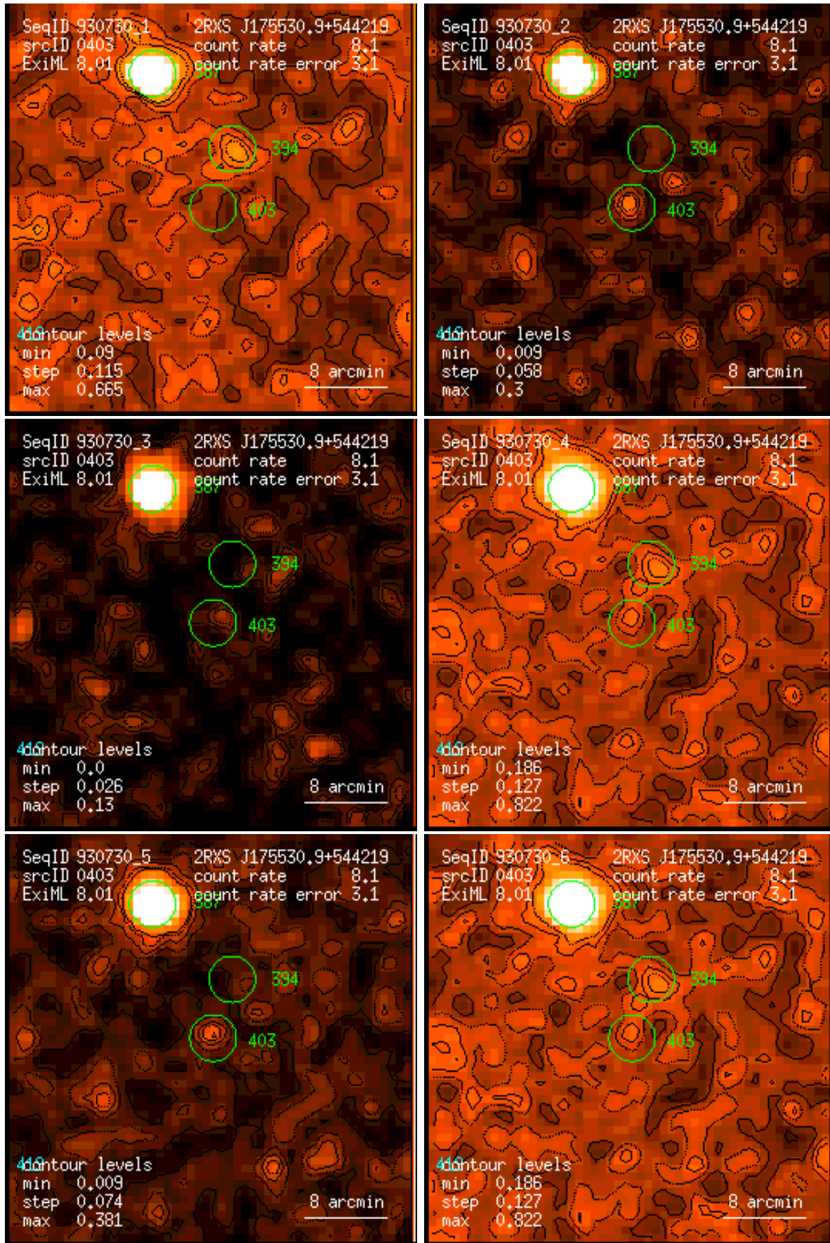
Figure 403: RASS 930730: detection 0403: band rate images, Gaussian filter: (1) PSPC channels 11 – 41, (2) 52 – 90, (3) 91 – 201, (4) 11 – 235, (5) 52 – 201, (6) 11 – 201. Broad band rates in counts/ks. Band rate contour levels in counts/ks/arcmin 2 .
