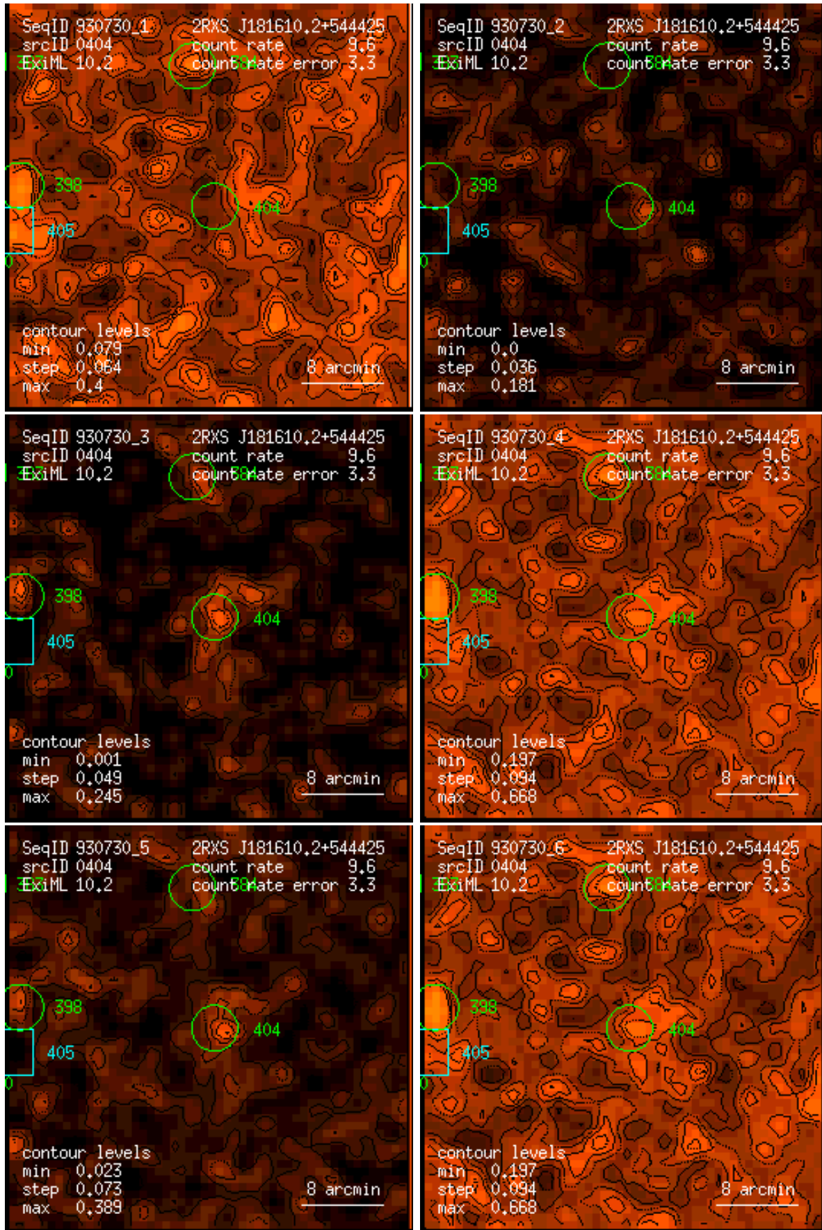
Figure 404: RASS 930730: detection 0404: band rate images, Gaussian filter: (1) PSPC channels 11 – 41, (2) 52 – 90, (3) 91 – 201, (4) 11 – 235, (5) 52 – 201, (6) 11 – 201. Broad band rates in counts/ks. Band rate contour levels in counts/ks/arcmin 2 .
