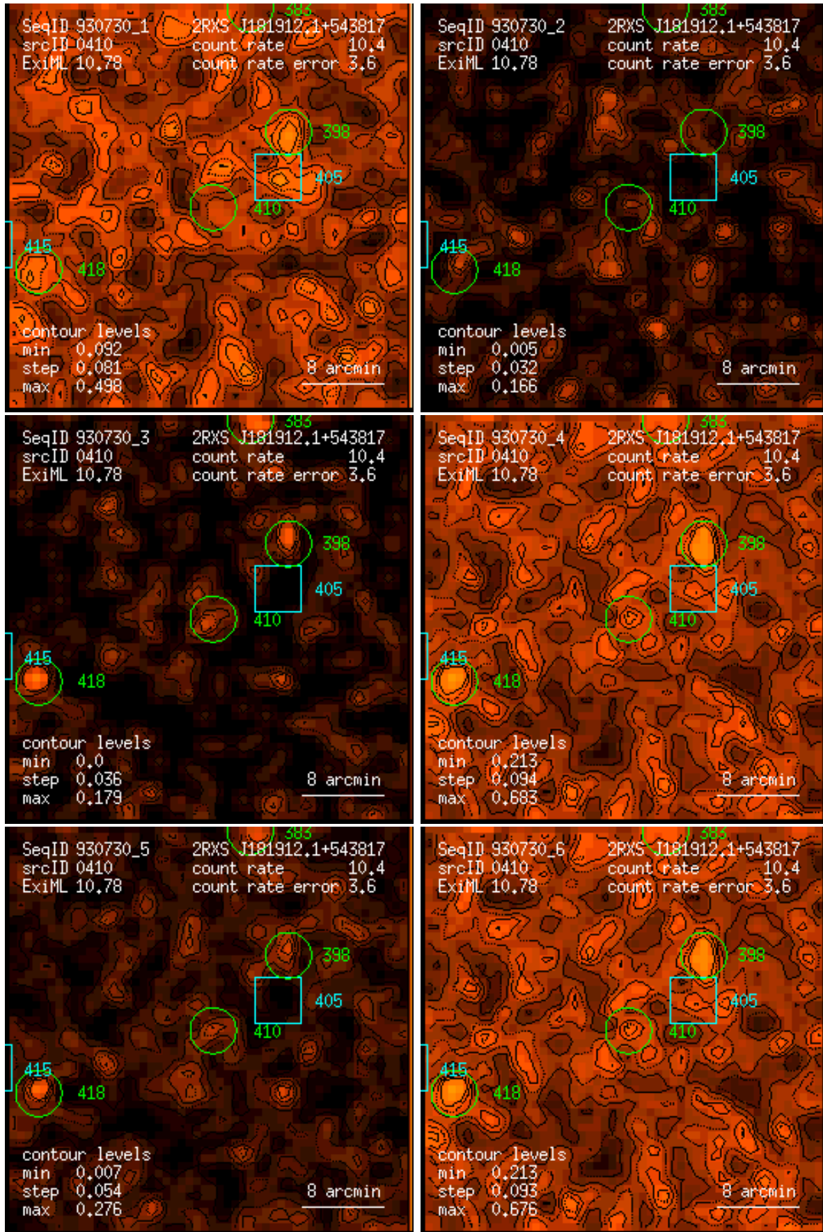
Figure 410: RASS 930730: detection 0410: band rate images, Gaussian filter: (1) PSPC channels 11 – 41, (2) 52 – 90, (3) 91 – 201, (4) 11 – 235, (5) 52 – 201, (6) 11 – 201. Broad band rates in counts/ks. Band rate contour levels in counts/ks/arcmin 2 .
