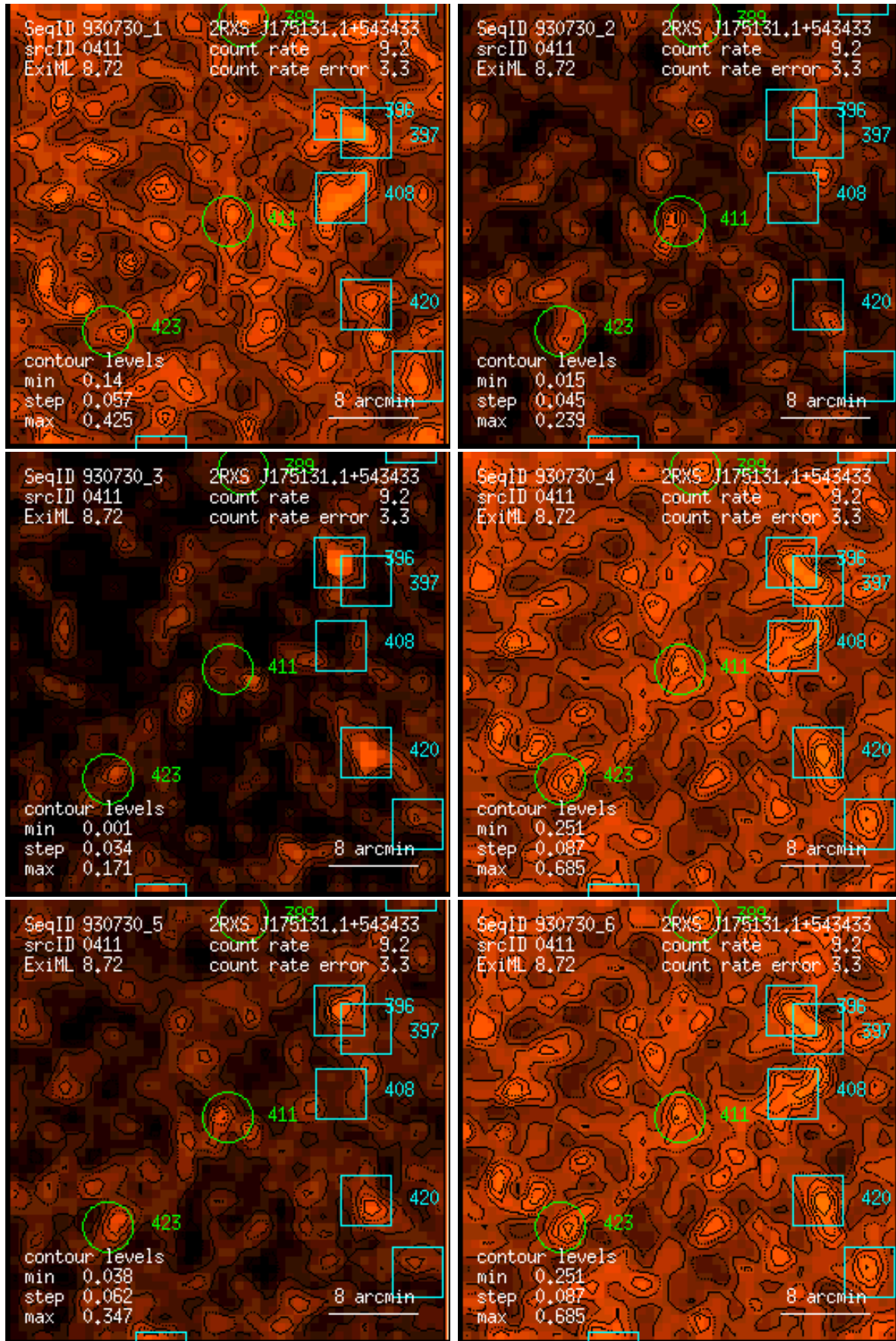
Figure 411: RASS 930730: detection 0411: band rate images, Gaussian filter: (1) PSPC channels 11 – 41, (2) 52 – 90, (3) 91 – 201, (4) 11 – 235, (5) 52 – 201, (6) 11 – 201. Broad band rates in counts/ks. Band rate contour levels in counts/ks/arcmin 2 .
