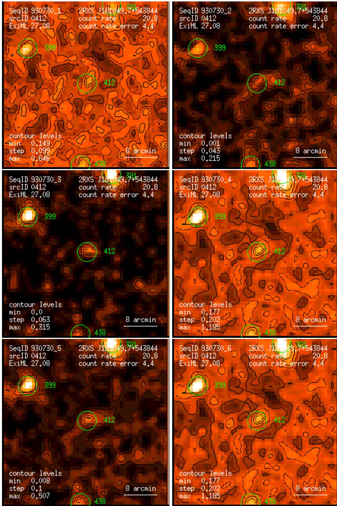
Figure 412: RASS 930730: detection 0412: band rate images, Gaussian filter: (1) PSPC channels 11 – 41, (2) 52 – 90, (3) 91 – 201, (4) 11 – 235, (5) 52 – 201, (6) 11 – 201. Broad band rates in counts/ks. Band rate contour levels in counts/ks/arcmin 2 .
