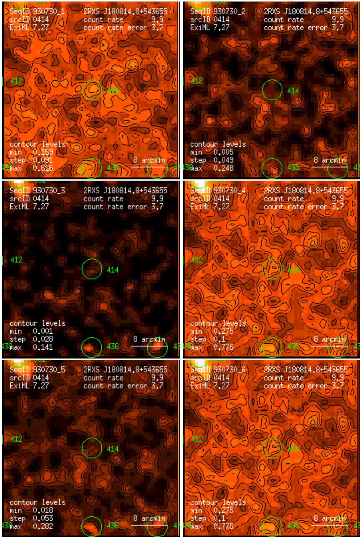
Figure 414: RASS 930730: detection 0414: band rate images, Gaussian filter: (1) PSPC channels 11 – 41, (2) 52 – 90, (3) 91 – 201, (4) 11 – 235, (5) 52 – 201, (6) 11 – 201. Broad band rates in counts/ks. Band rate contour levels in counts/ks/arcmin 2 .
