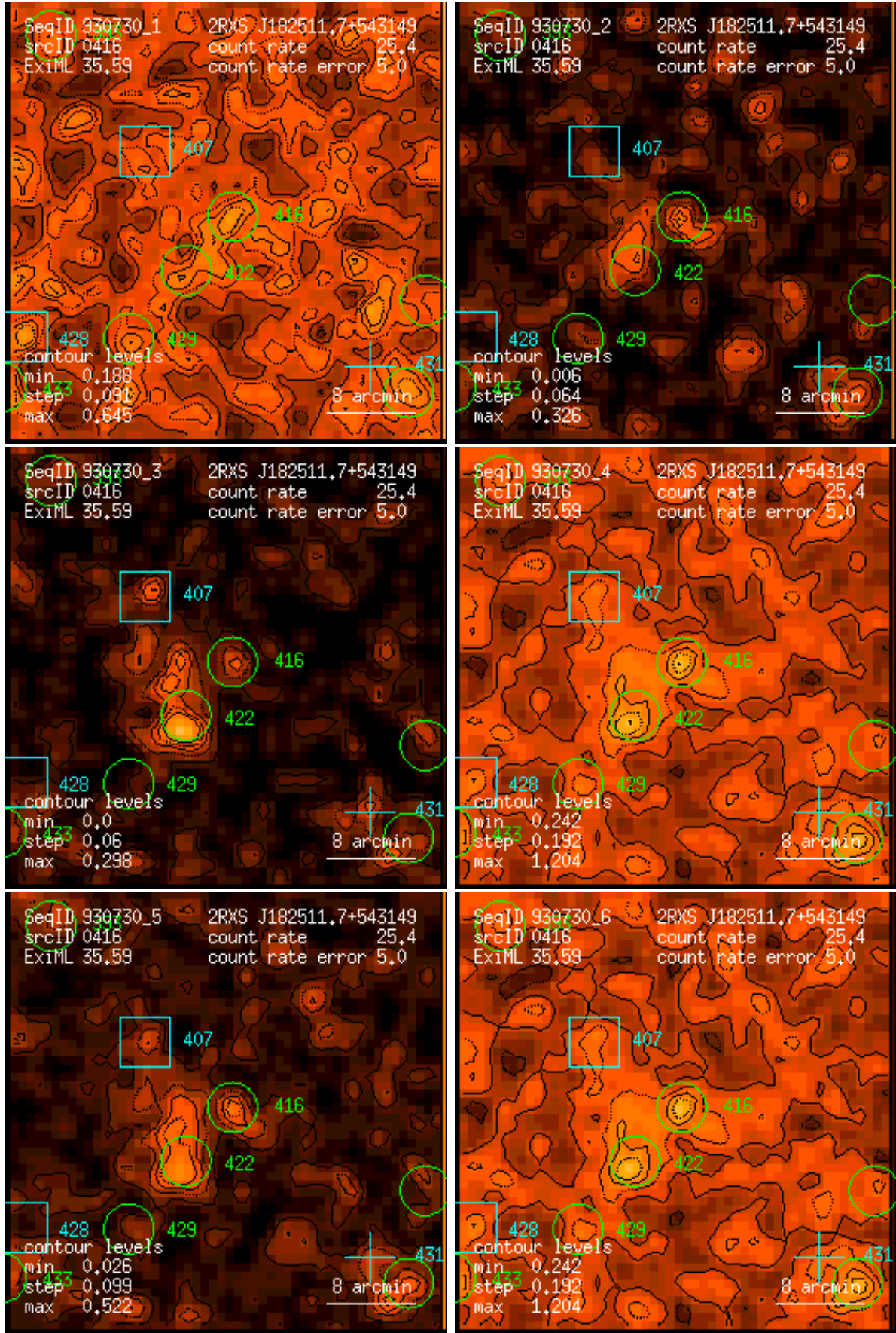
Figure 416: RASS 930730: detection 0416: band rate images, Gaussian filter: (1) PSPC channels 11 – 41, (2) 52 – 90, (3) 91 – 201, (4) 11 – 235, (5) 52 – 201, (6) 11 – 201. Broad band rates in counts/ks. Band rate contour levels in counts/ks/arcmin 2 .
