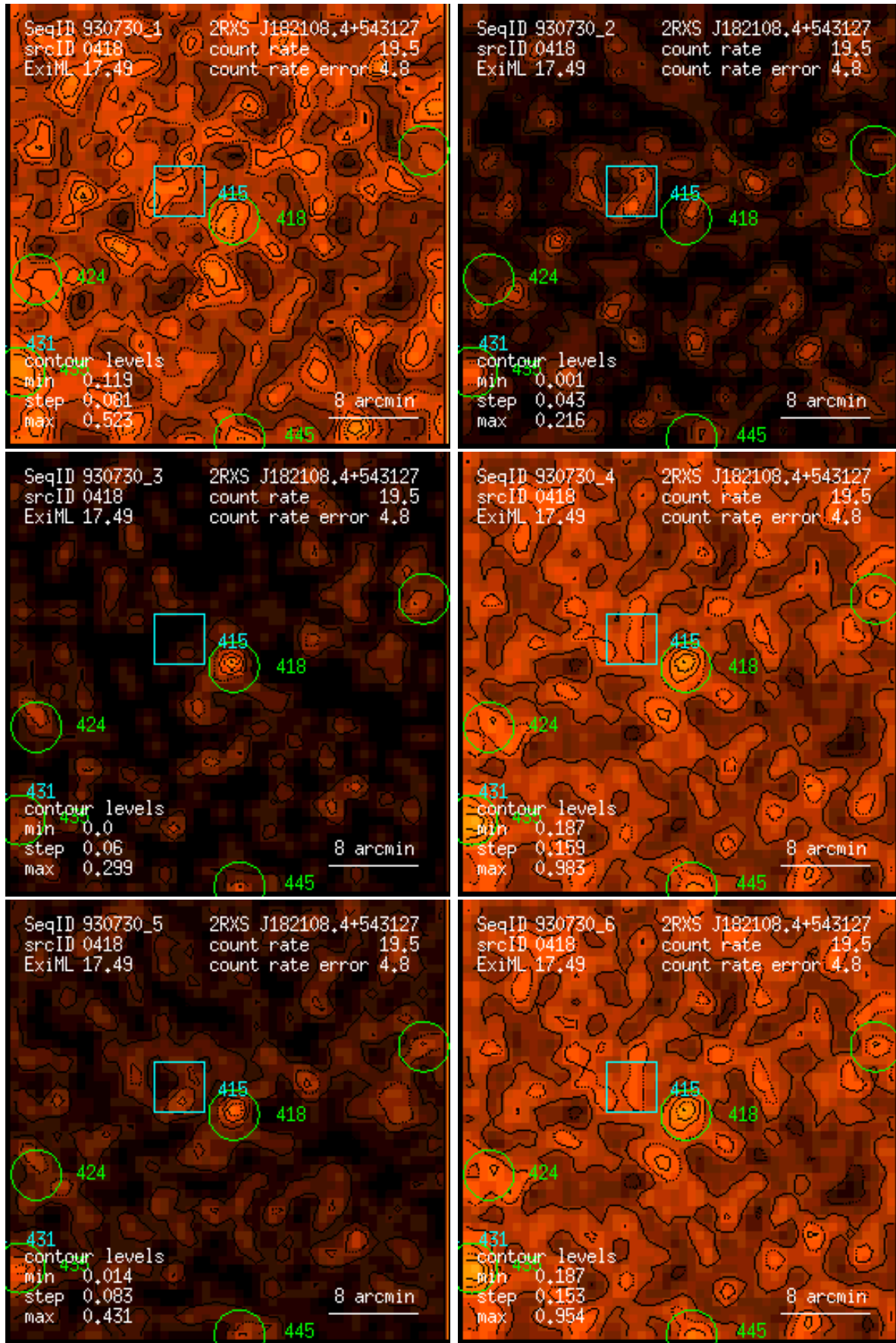
Figure 418: RASS 930730: detection 0418: band rate images, Gaussian filter: (1) PSPC channels 11 – 41, (2) 52 – 90, (3) 91 – 201, (4) 11 – 235, (5) 52 – 201, (6) 11 – 201. Broad band rates in counts/ks. Band rate contour levels in counts/ks/arcmin 2 .
