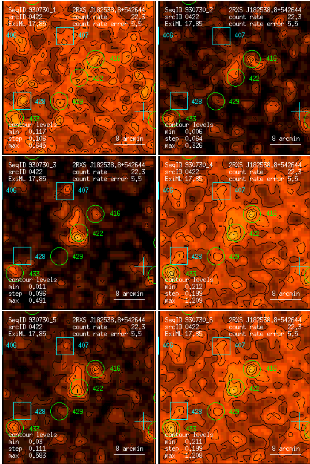
Figure 422: RASS 930730: detection 0422: band rate images, Gaussian filter: (1) PSPC channels 11 – 41, (2) 52 – 90, (3) 91 – 201, (4) 11 – 235, (5) 52 – 201, (6) 11 – 201. Broad band rates in counts/ks. Band rate contour levels in counts/ks/arcmin 2 .
