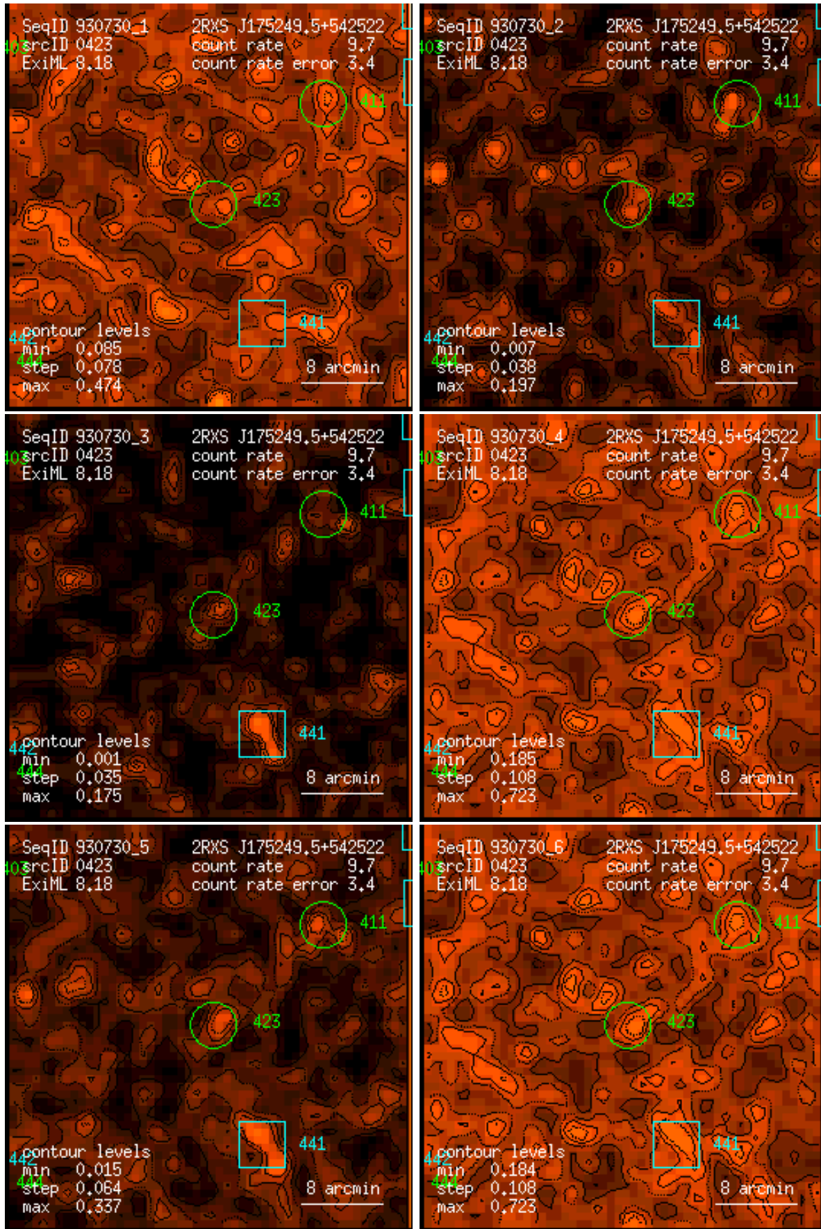
Figure 423: RASS 930730: detection 0423: band rate images, Gaussian filter: (1) PSPC channels 11 – 41, (2) 52 – 90, (3) 91 – 201, (4) 11 – 235, (5) 52 – 201, (6) 11 – 201. Broad band rates in counts/ks. Band rate contour levels in counts/ks/arcmin 2 .
