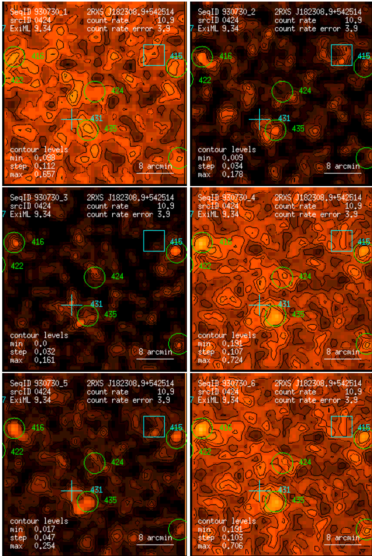
Figure 424: RASS 930730: detection 0424: band rate images, Gaussian filter: (1) PSPC channels 11 – 41, (2) 52 – 90, (3) 91 – 201, (4) 11 – 235, (5) 52 – 201, (6) 11 – 201. Broad band rates in counts/ks. Band rate contour levels in counts/ks/arcmin 2 .
