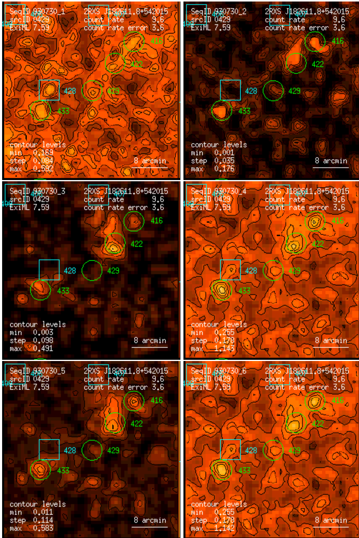
Figure 429: RASS 930730: detection 0429: band rate images, Gaussian filter: (1) PSPC channels 11 – 41, (2) 52 – 90, (3) 91 – 201, (4) 11 – 235, (5) 52 – 201, (6) 11 – 201. Broad band rates in counts/ks. Band rate contour levels in counts/ks/arcmin 2 .
