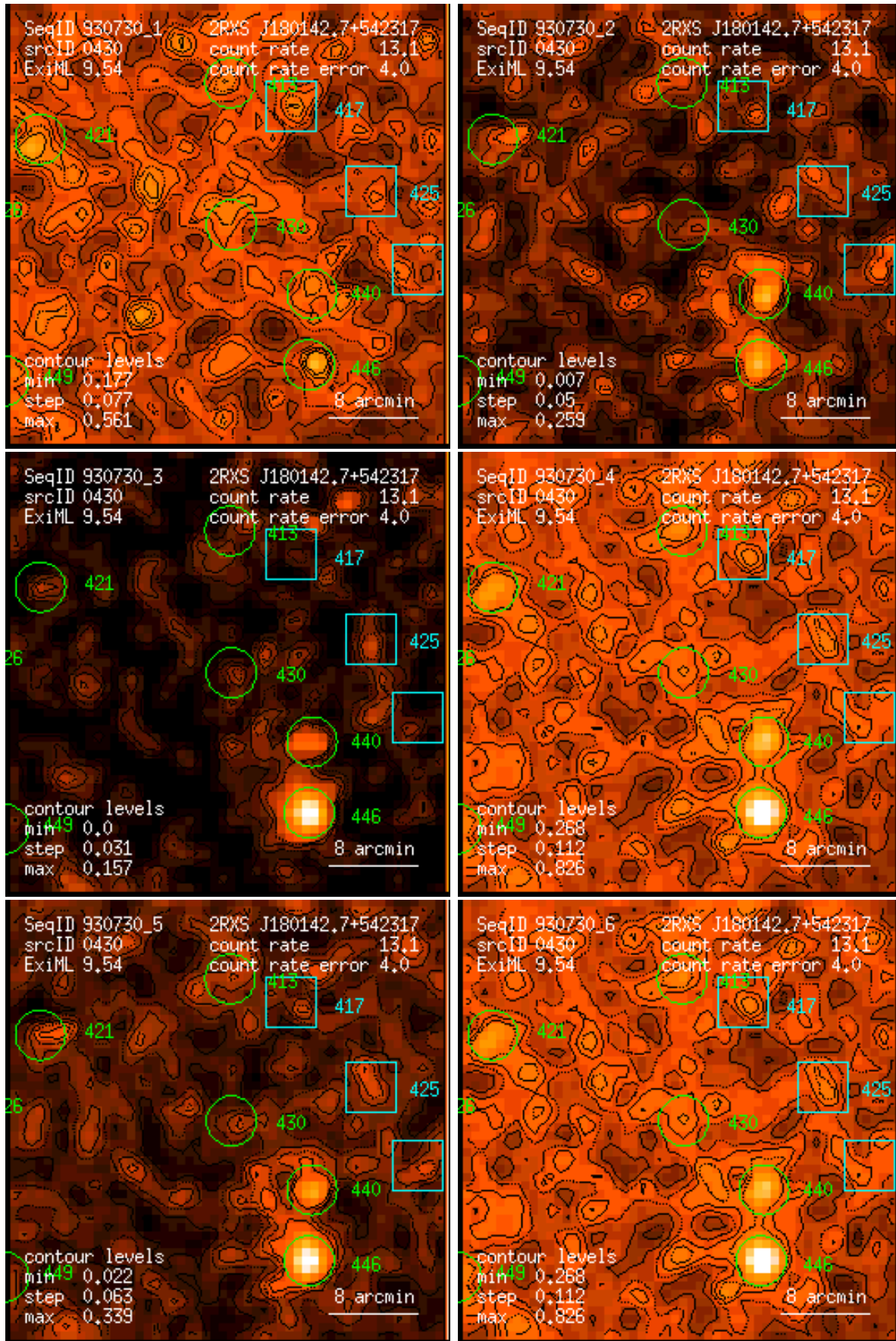
Figure 430: RASS 930730: detection 0430: band rate images, Gaussian filter: (1) PSPC channels 11 – 41, (2) 52 – 90, (3) 91 – 201, (4) 11 – 235, (5) 52 – 201, (6) 11 – 201. Broad band rates in counts/ks. Band rate contour levels in counts/ks/arcmin 2 .
