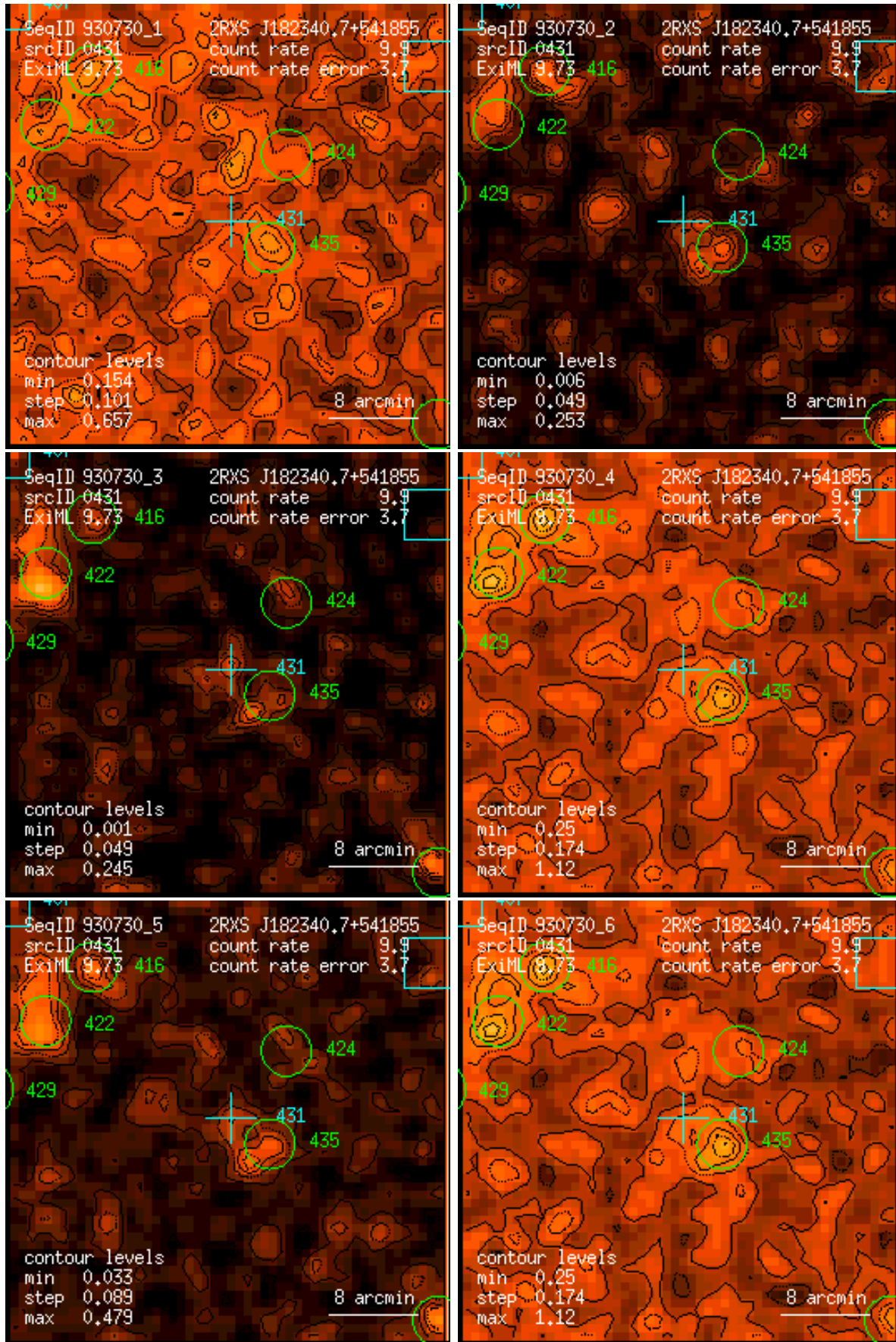
Figure 431: RASS 930730: detection 0431: band rate images, Gaussian filter: (1) PSPC channels 11 – 41, (2) 52 – 90, (3) 91 – 201, (4) 11 – 235, (5) 52 – 201, (6) 11 – 201. Broad band rates in counts/ks. Band rate contour levels in counts/ks/arcmin 2 .
