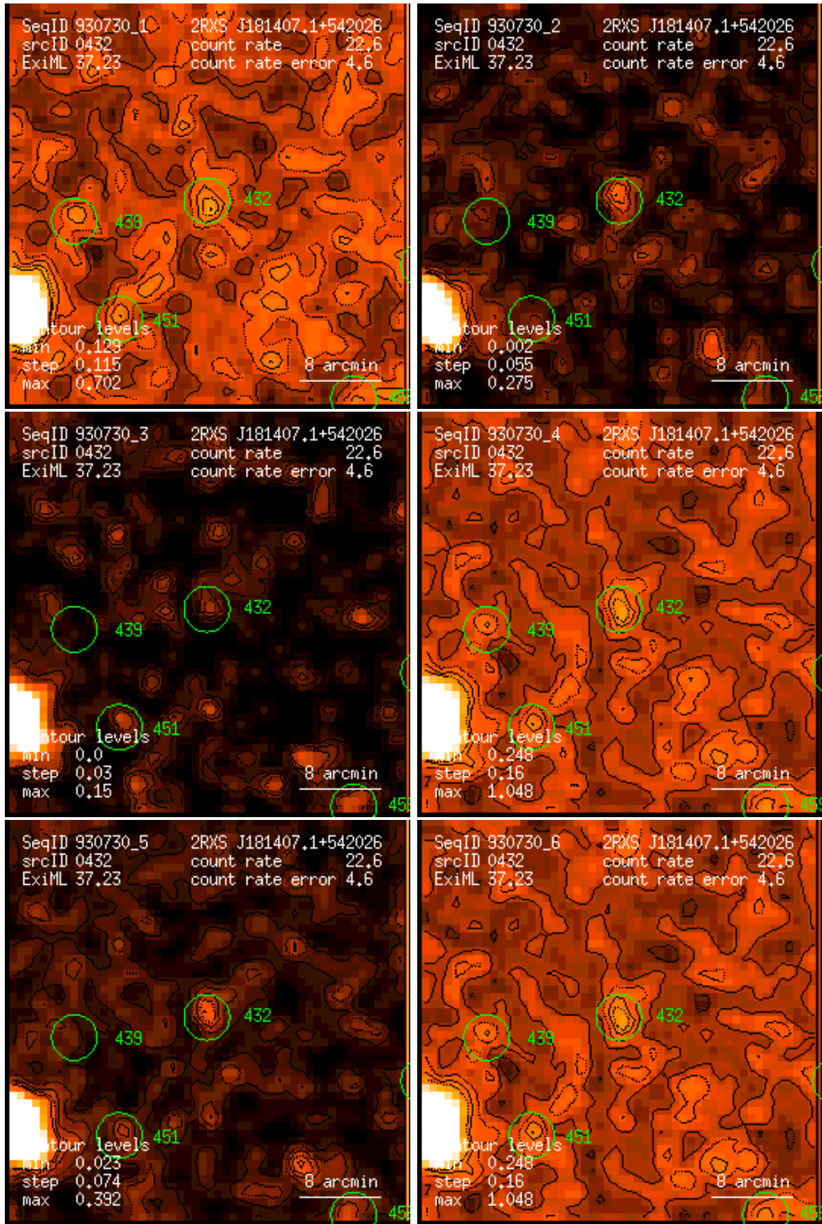
Figure 432: RASS 930730: detection 0432: band rate images, Gaussian filter: (1) PSPC channels 11 – 41, (2) 52 – 90, (3) 91 – 201, (4) 11 – 235, (5) 52 – 201, (6) 11 – 201. Broad band rates in counts/ks. Band rate contour levels in counts/ks/arcmin 2 .
