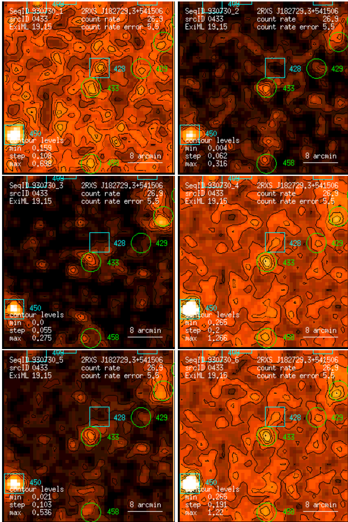
Figure 433: RASS 930730: detection 0433: band rate images, Gaussian filter: (1) PSPC channels 11 – 41, (2) 52 – 90, (3) 91 – 201, (4) 11 – 235, (5) 52 – 201, (6) 11 – 201. Broad band rates in counts/ks. Band rate contour levels in counts/ks/arcmin 2 .
