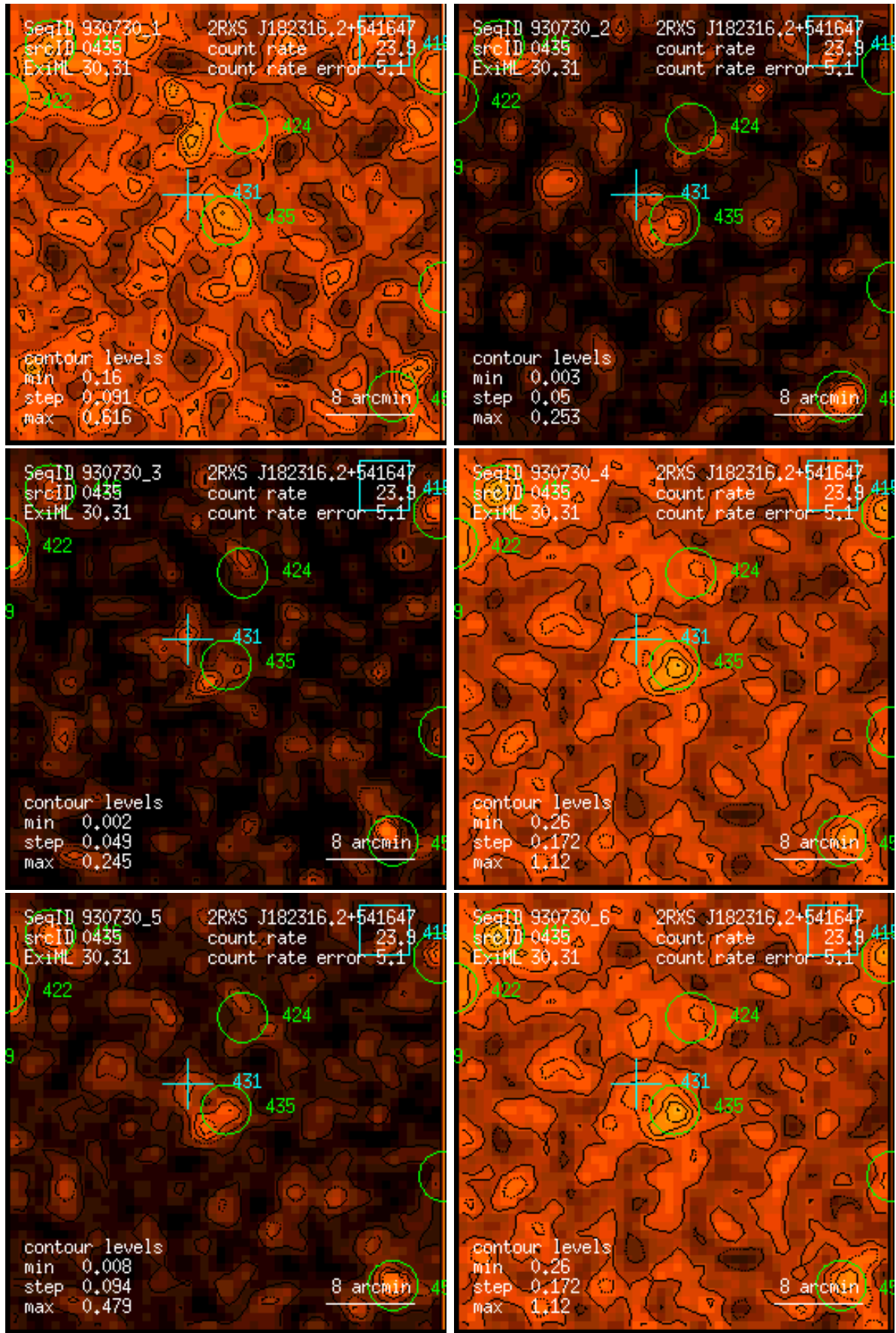
Figure 435: RASS 930730: detection 0435: band rate images, Gaussian filter: (1) PSPC channels 11 – 41, (2) 52 – 90, (3) 91 – 201, (4) 11 – 235, (5) 52 – 201, (6) 11 – 201. Broad band rates in counts/ks. Band rate contour levels in counts/ks/arcmin 2 .
