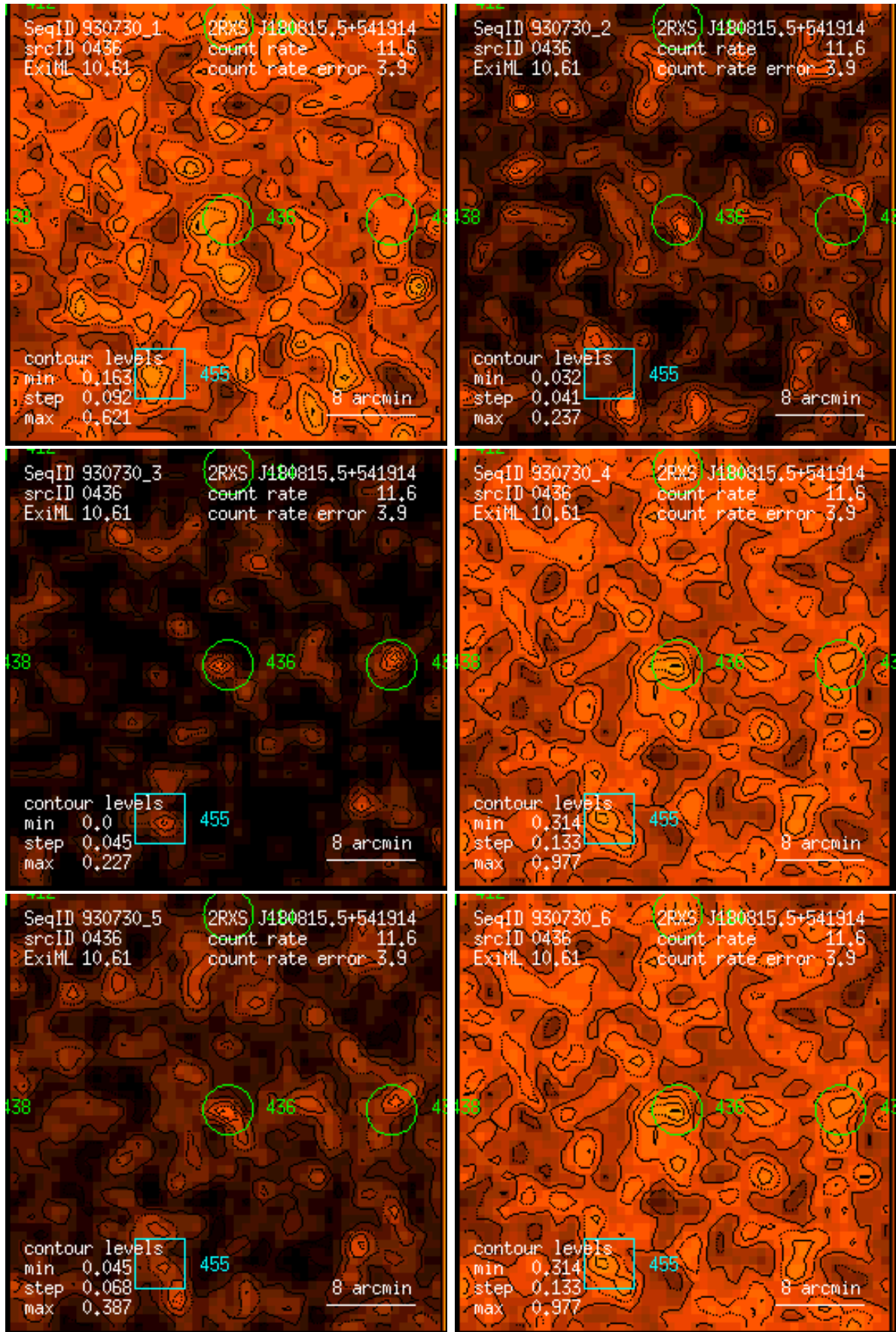
Figure 436: RASS 930730: detection 0436: band rate images, Gaussian filter: (1) PSPC channels 11 – 41, (2) 52 – 90, (3) 91 – 201, (4) 11 – 235, (5) 52 – 201, (6) 11 – 201. Broad band rates in counts/ks. Band rate contour levels in counts/ks/arcmin 2 .
