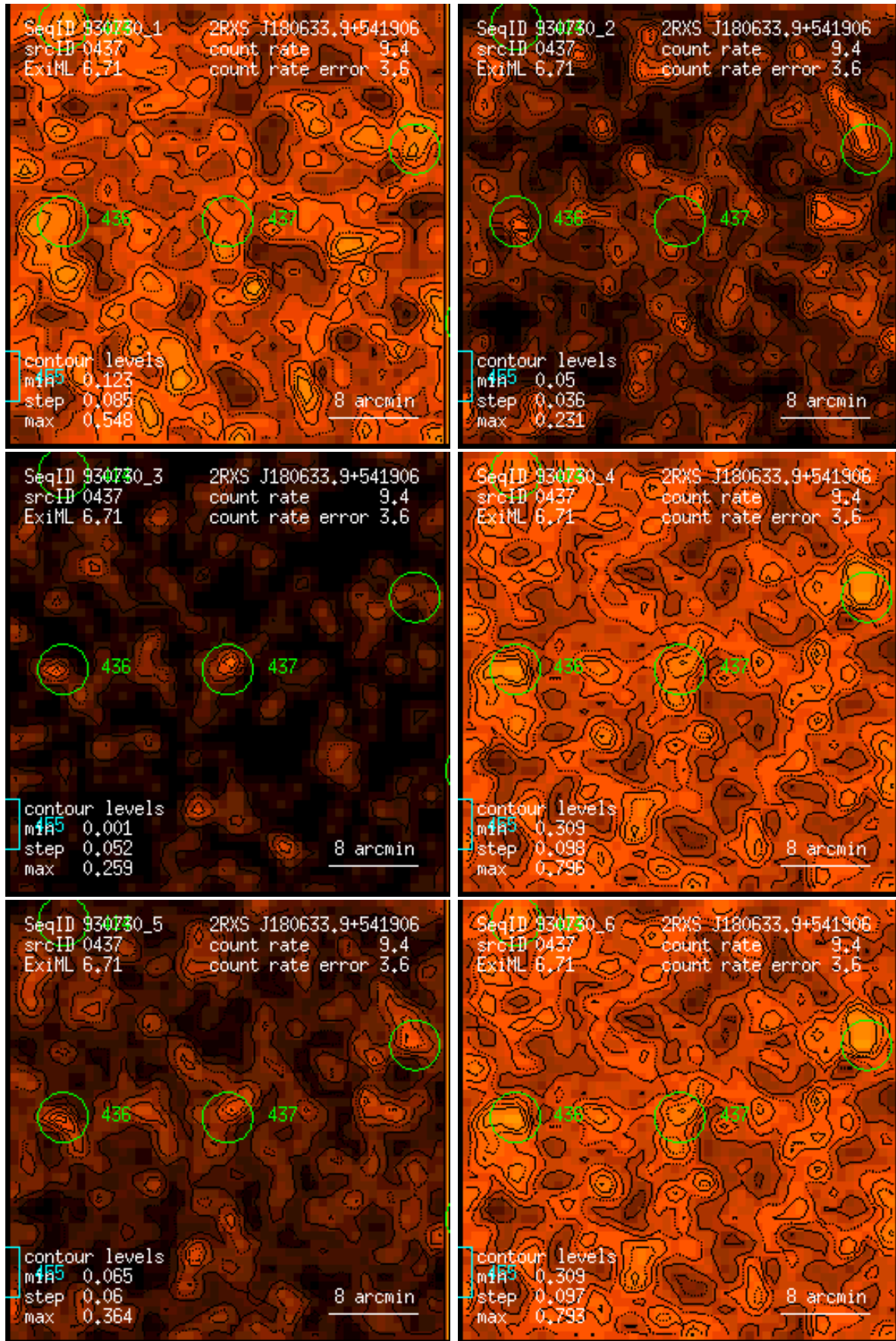
Figure 437: RASS 930730: detection 0437: band rate images, Gaussian filter: (1) PSPC channels 11 – 41, (2) 52 – 90, (3) 91 – 201, (4) 11 – 235, (5) 52 – 201, (6) 11 – 201. Broad band rates in counts/ks. Band rate contour levels in counts/ks/arcmin 2 .
