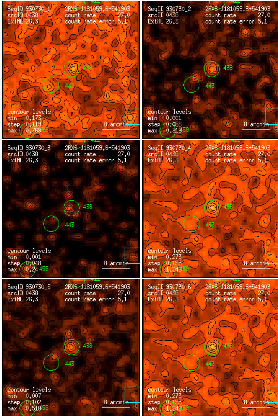
Figure 438: RASS 930730: detection 0438: band rate images, Gaussian filter: (1) PSPC channels 11 – 41, (2) 52 – 90, (3) 91 – 201, (4) 11 – 235, (5) 52 – 201, (6) 11 – 201. Broad band rates in counts/ks. Band rate contour levels in counts/ks/arcmin 2 .
