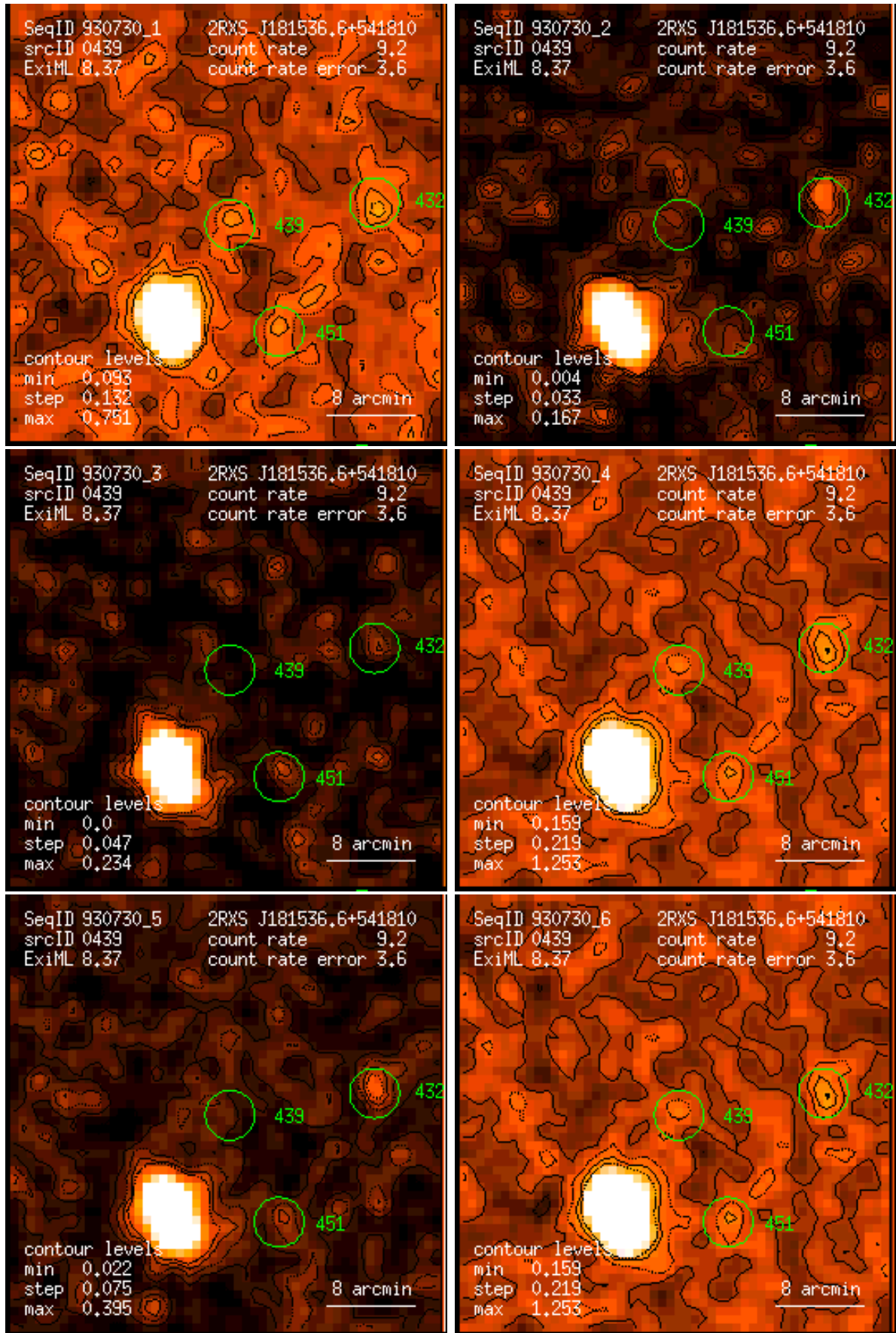
Figure 439: RASS 930730: detection 0439: band rate images, Gaussian filter: (1) PSPC channels 11 – 41, (2) 52 – 90, (3) 91 – 201, (4) 11 – 235, (5) 52 – 201, (6) 11 – 201. Broad band rates in counts/ks. Band rate contour levels in counts/ks/arcmin 2 .
