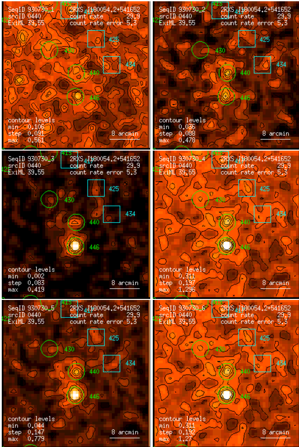
Figure 440: RASS 930730: detection 0440: band rate images, Gaussian filter: (1) PSPC channels 11 – 41, (2) 52 – 90, (3) 91 – 201, (4) 11 – 235, (5) 52 – 201, (6) 11 – 201. Broad band rates in counts/ks. Band rate contour levels in counts/ks/arcmin 2 .
