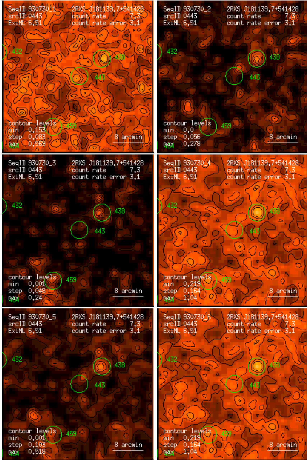
Figure 443: RASS 930730: detection 0443: band rate images, Gaussian filter: (1) PSPC channels 11 – 41, (2) 52 – 90, (3) 91 – 201, (4) 11 – 235, (5) 52 – 201, (6) 11 – 201. Broad band rates in counts/ks. Band rate contour levels in counts/ks/arcmin 2 .
