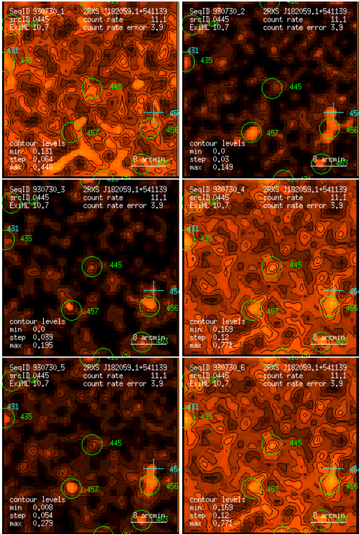
Figure 445: RASS 930730: detection 0445: band rate images, Gaussian filter: (1) PSPC channels 11 – 41, (2) 52 – 90, (3) 91 – 201, (4) 11 – 235, (5) 52 – 201, (6) 11 – 201. Broad band rates in counts/ks. Band rate contour levels in counts/ks/arcmin 2 .
