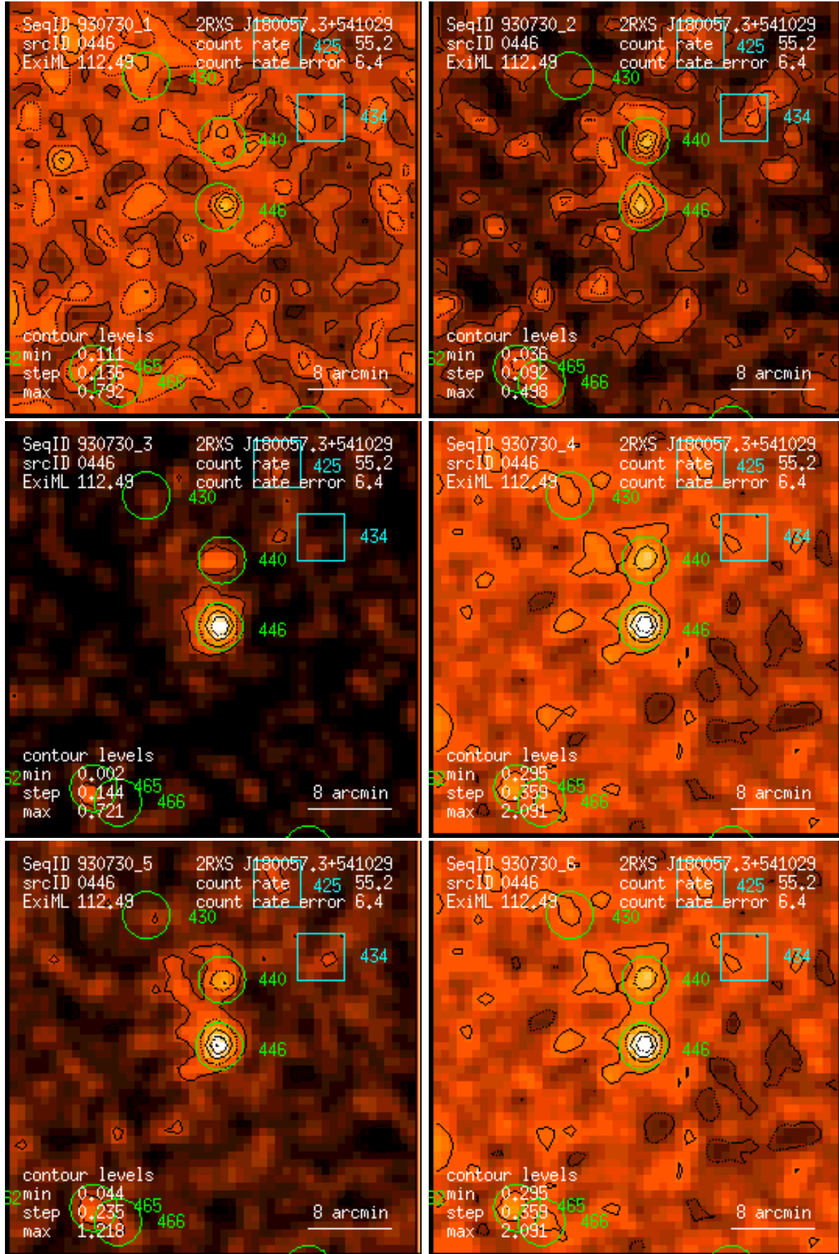
Figure 446: RASS 930730: detection 0446: band rate images, Gaussian filter: (1) PSPC channels 11 – 41, (2) 52 – 90, (3) 91 – 201, (4) 11 – 235, (5) 52 – 201, (6) 11 – 201. Broad band rates in counts/ks. Band rate contour levels in counts/ks/arcmin 2 .
