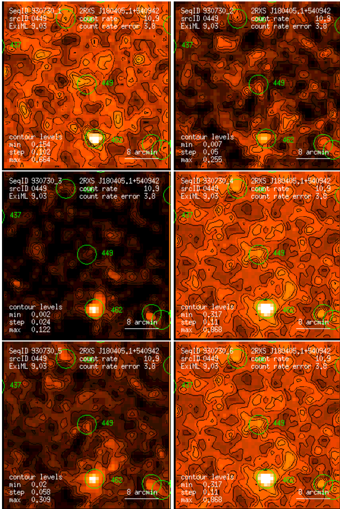
Figure 449: RASS 930730: detection 0449: band rate images, Gaussian filter: (1) PSPC channels 11 – 41, (2) 52 – 90, (3) 91 – 201, (4) 11 – 235, (5) 52 – 201, (6) 11 – 201. Broad band rates in counts/ks. Band rate contour levels in counts/ks/arcmin 2 .
