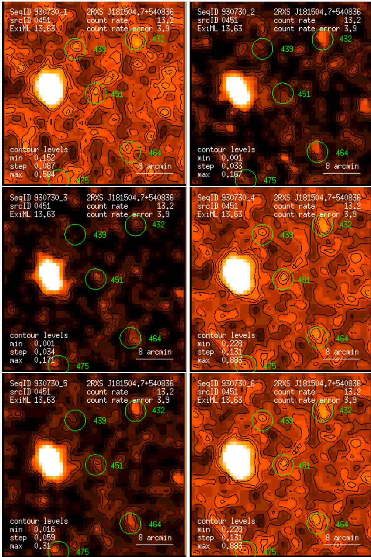
Figure 451: RASS 930730: detection 0451: band rate images, Gaussian filter: (1) PSPC channels 11 – 41, (2) 52 – 90, (3) 91 – 201, (4) 11 – 235, (5) 52 – 201, (6) 11 – 201. Broad band rates in counts/ks. Band rate contour levels in counts/ks/arcmin 2 .
