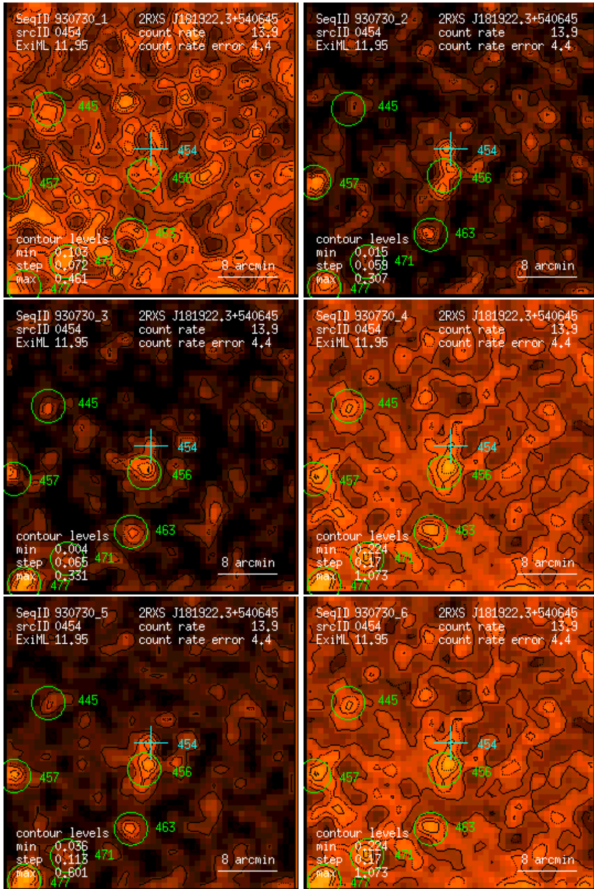
Figure 454: RASS 930730: detection 0454: band rate images, Gaussian filter: (1) PSPC channels 11 – 41, (2) 52 – 90, (3) 91 – 201, (4) 11 – 235, (5) 52 – 201, (6) 11 – 201. Broad band rates in counts/ks. Band rate contour levels in counts/ks/arcmin 2 .
