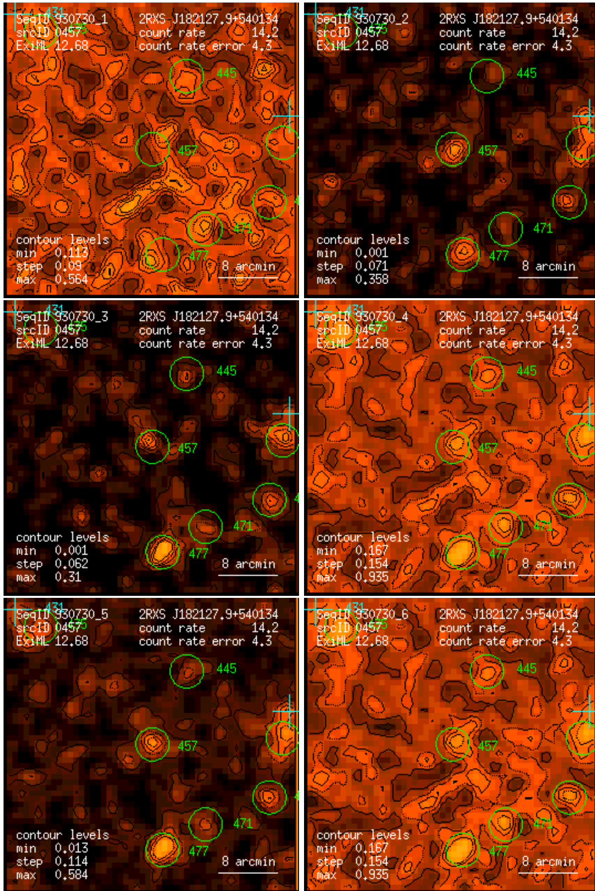
Figure 457: RASS 930730: detection 0457: band rate images, Gaussian filter: (1) PSPC channels 11 – 41, (2) 52 – 90, (3) 91 – 201, (4) 11 – 235, (5) 52 – 201, (6) 11 – 201. Broad band rates in counts/ks. Band rate contour levels in counts/ks/arcmin 2 .
