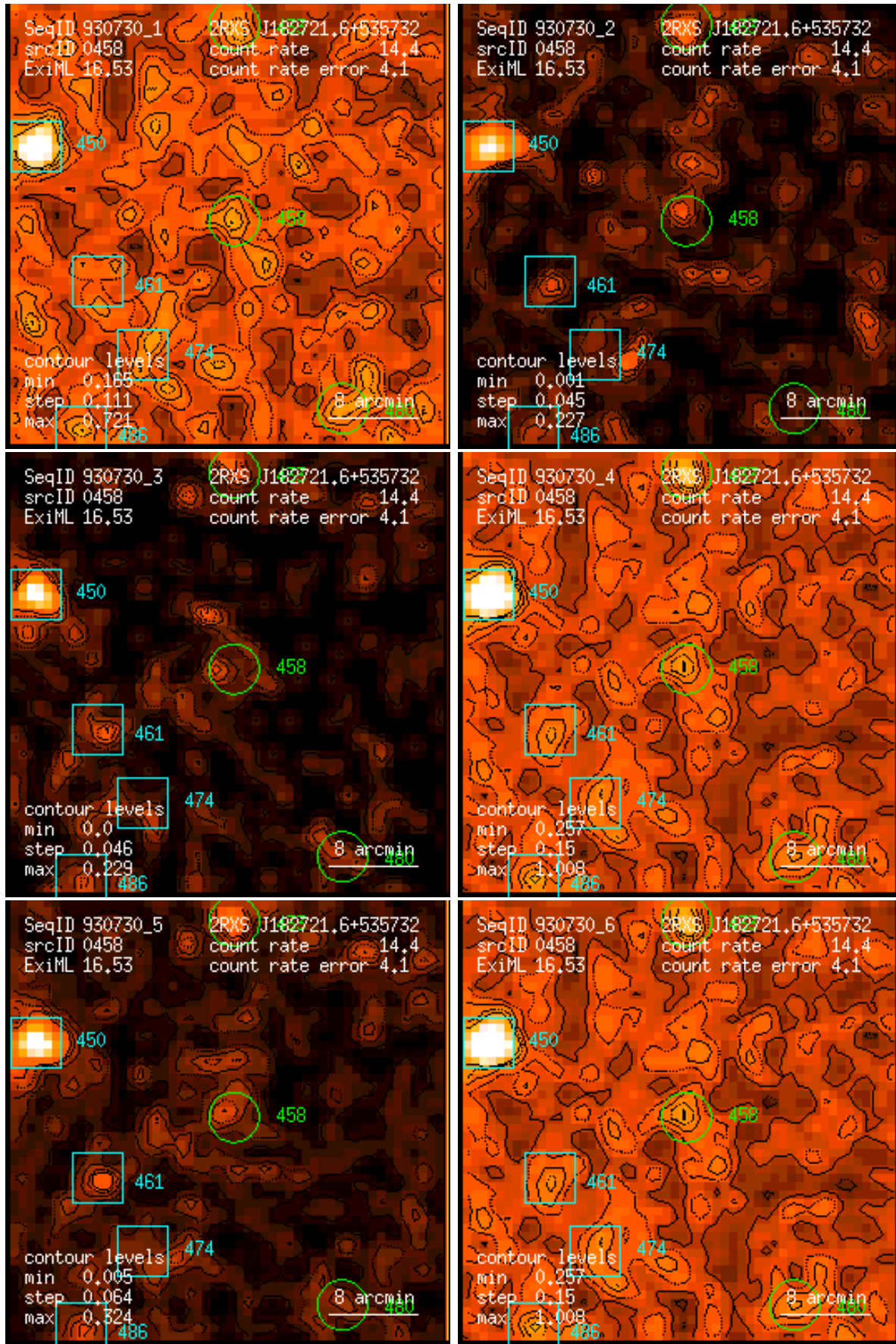
Figure 458: RASS 930730: detection 0458: band rate images, Gaussian filter: (1) PSPC channels 11 – 41, (2) 52 – 90, (3) 91 – 201, (4) 11 – 235, (5) 52 – 201, (6) 11 – 201. Broad band rates in counts/ks. Band rate contour levels in counts/ks/arcmin 2 .
