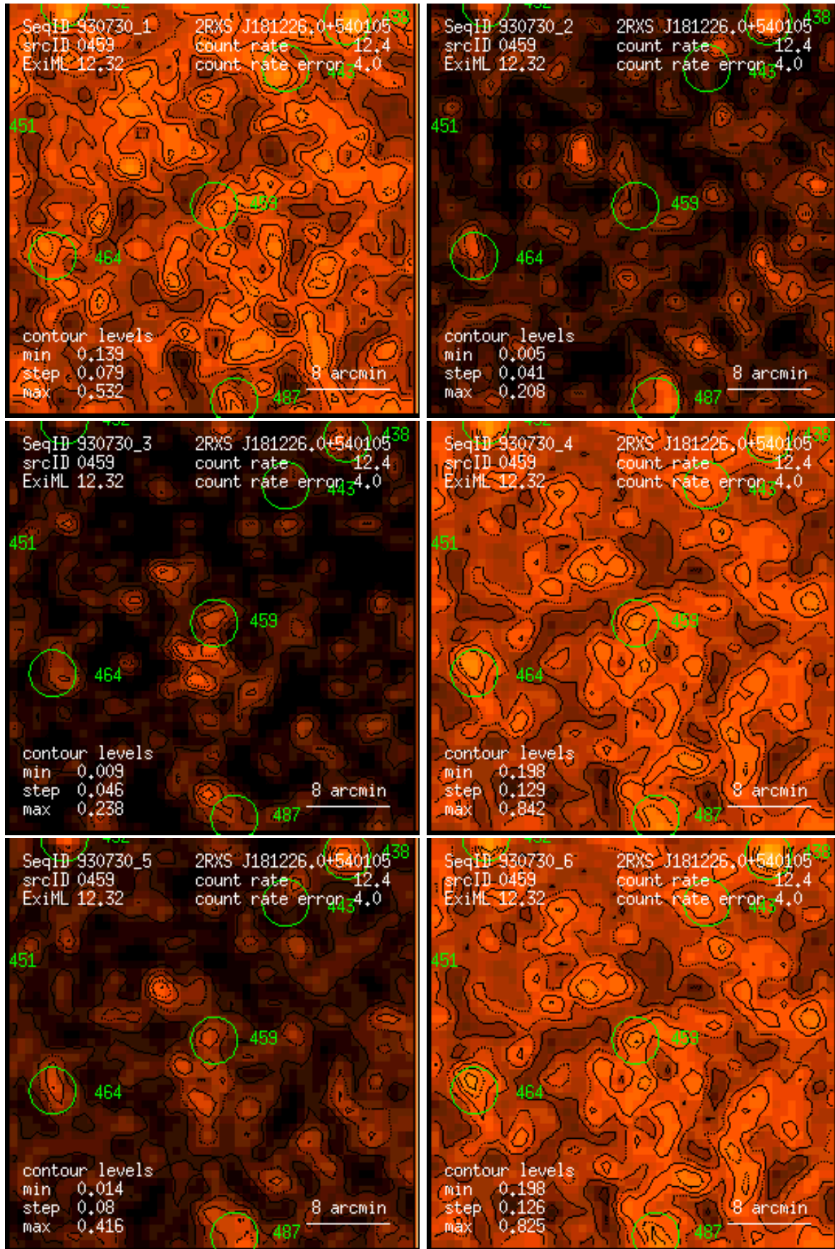
Figure 459: RASS 930730: detection 0459: band rate images, Gaussian filter: (1) PSPC channels 11 – 41, (2) 52 – 90, (3) 91 – 201, (4) 11 – 235, (5) 52 – 201, (6) 11 – 201. Broad band rates in counts/ks. Band rate contour levels in counts/ks/arcmin 2 .
