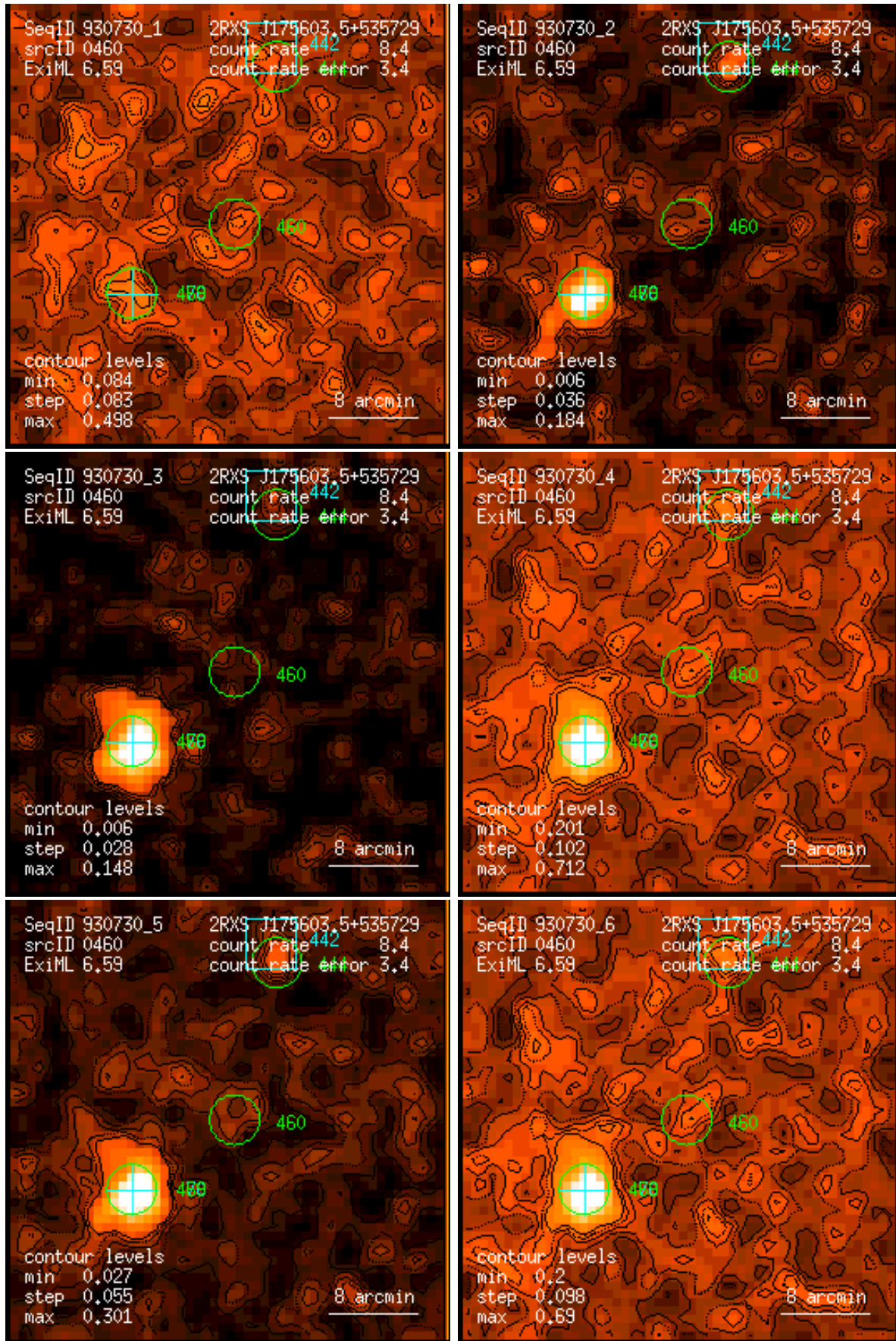
Figure 460: RASS 930730: detection 0460: band rate images, Gaussian filter: (1) PSPC channels 11 – 41, (2) 52 – 90, (3) 91 – 201, (4) 11 – 235, (5) 52 – 201, (6) 11 – 201. Broad band rates in counts/ks. Band rate contour levels in counts/ks/arcmin 2 .
