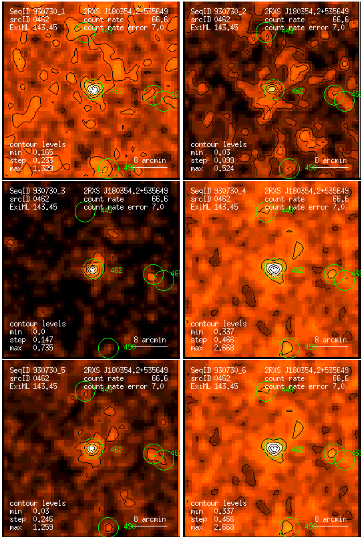
Figure 462: RASS 930730: detection 0462: band rate images, Gaussian filter: (1) PSPC channels 11 – 41, (2) 52 – 90, (3) 91 – 201, (4) 11 – 235, (5) 52 – 201, (6) 11 – 201. Broad band rates in counts/ks. Band rate contour levels in counts/ks/arcmin 2 .
