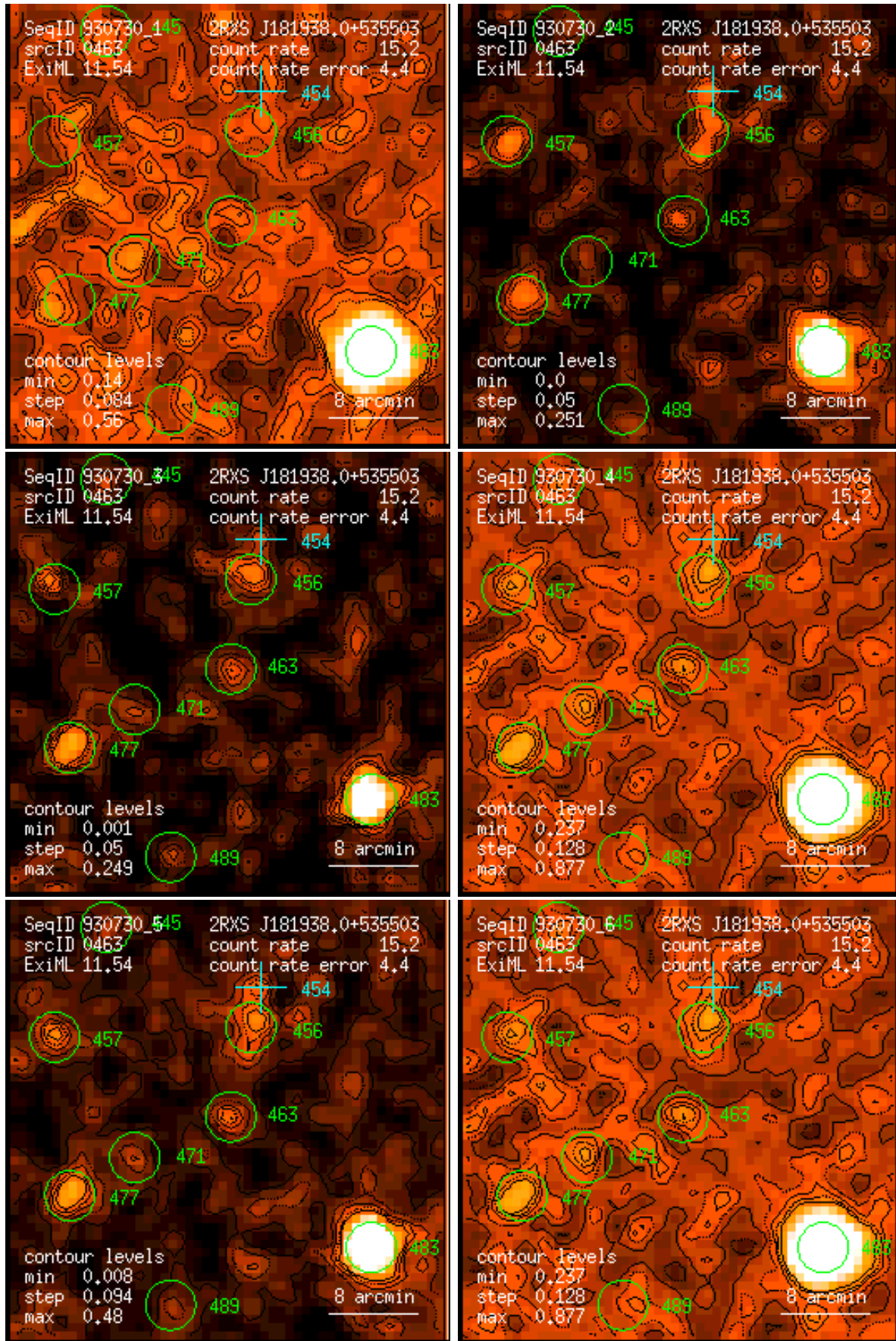
Figure 463: RASS 930730: detection 0463: band rate images, Gaussian filter: (1) PSPC channels 11 – 41, (2) 52 – 90, (3) 91 – 201, (4) 11 – 235, (5) 52 – 201, (6) 11 – 201. Broad band rates in counts/ks. Band rate contour levels in counts/ks/arcmin 2 .
