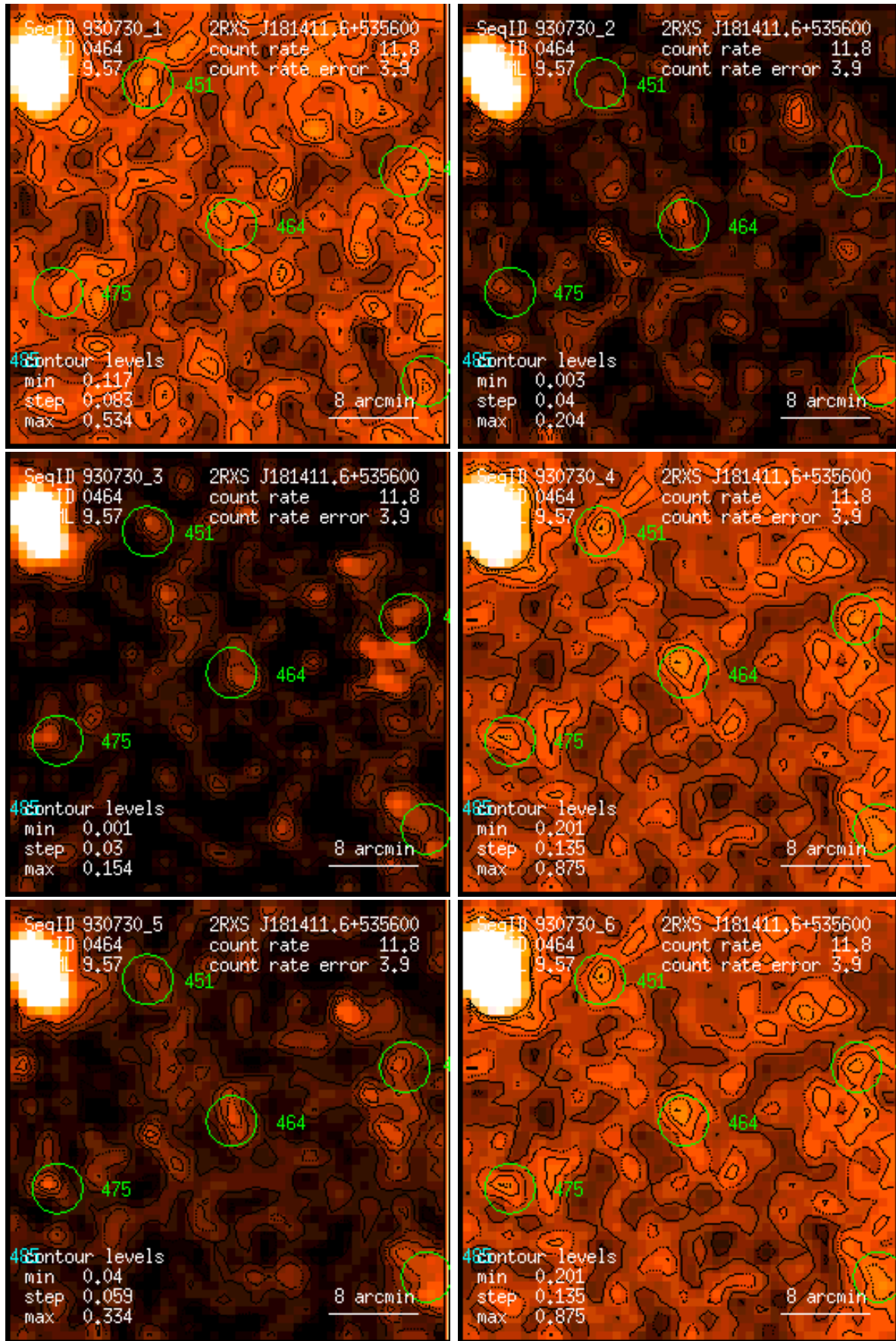
Figure 464: RASS 930730: detection 0464: band rate images, Gaussian filter: (1) PSPC channels 11 – 41, (2) 52 – 90, (3) 91 – 201, (4) 11 – 235, (5) 52 – 201, (6) 11 – 201. Broad band rates in counts/ks. Band rate contour levels in counts/ks/arcmin 2 .
