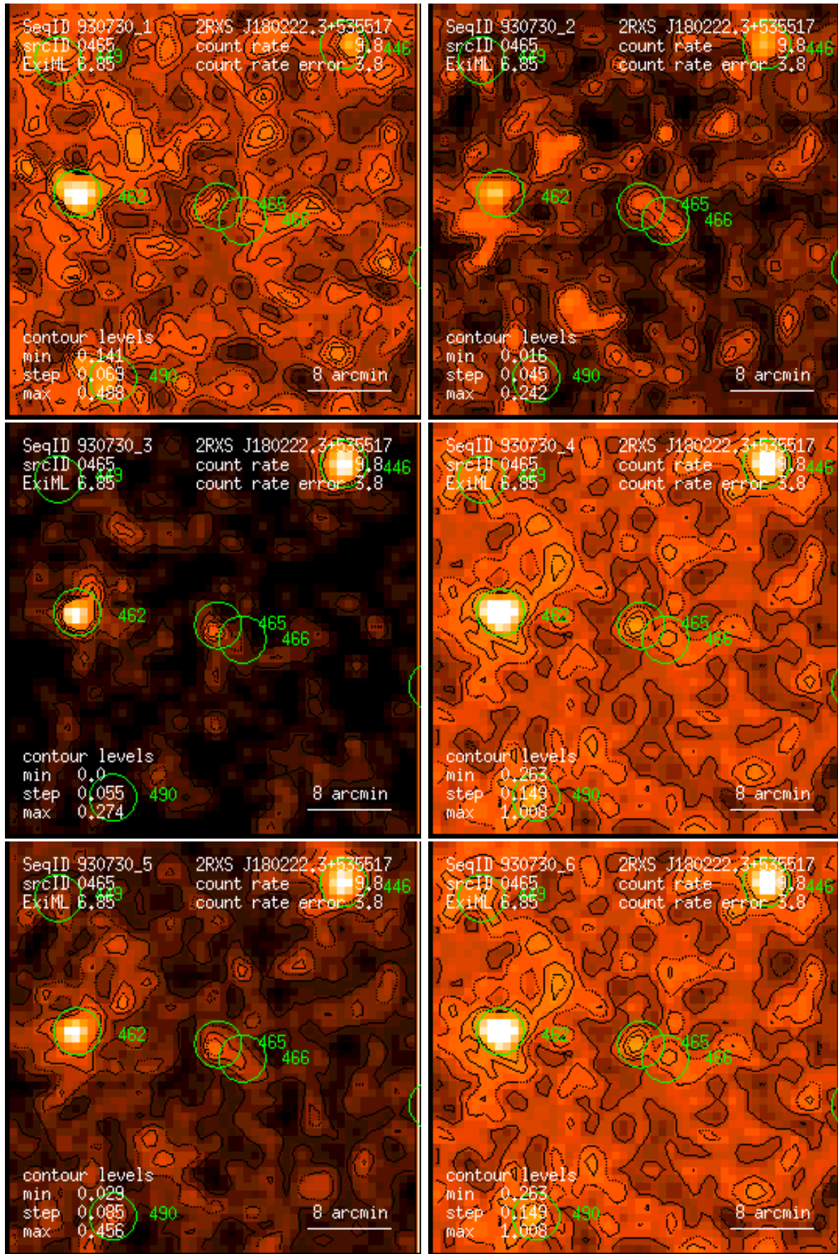
Figure 465: RASS 930730: detection 0465: band rate images, Gaussian filter: (1) PSPC channels 11 – 41, (2) 52 – 90, (3) 91 – 201, (4) 11 – 235, (5) 52 – 201, (6) 11 – 201. Broad band rates in counts/ks. Band rate contour levels in counts/ks/arcmin 2 .
