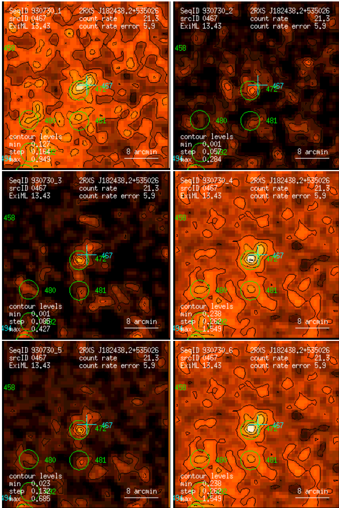
Figure 467: RASS 930730: detection 0467: band rate images, Gaussian filter: (1) PSPC channels 11 – 41, (2) 52 – 90, (3) 91 – 201, (4) 11 – 235, (5) 52 – 201, (6) 11 – 201. Broad band rates in counts/ks. Band rate contour levels in counts/ks/arcmin 2 .
