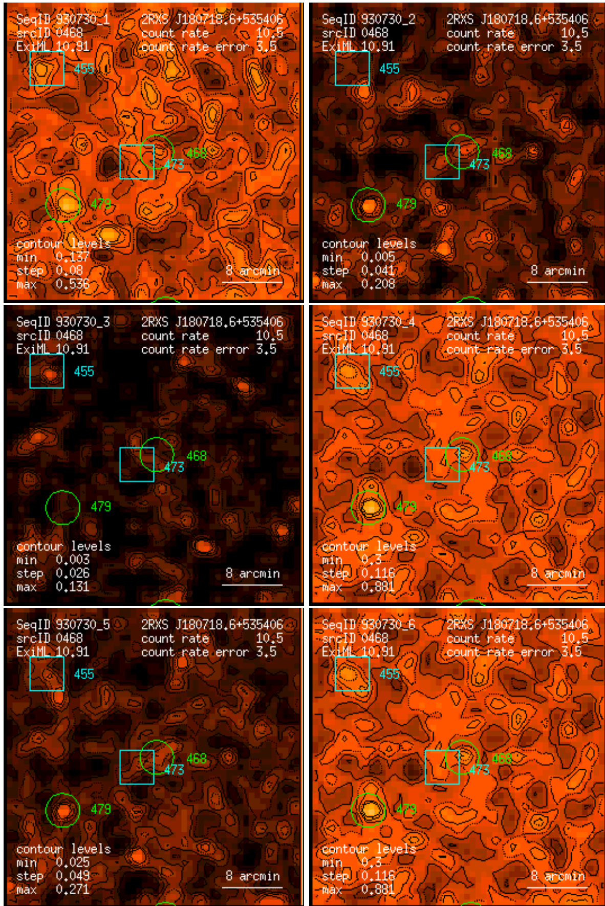
Figure 468: RASS 930730: detection 0468: band rate images, Gaussian filter: (1) PSPC channels 11 – 41, (2) 52 – 90, (3) 91 – 201, (4) 11 – 235, (5) 52 – 201, (6) 11 – 201. Broad band rates in counts/ks. Band rate contour levels in counts/ks/arcmin 2 .
