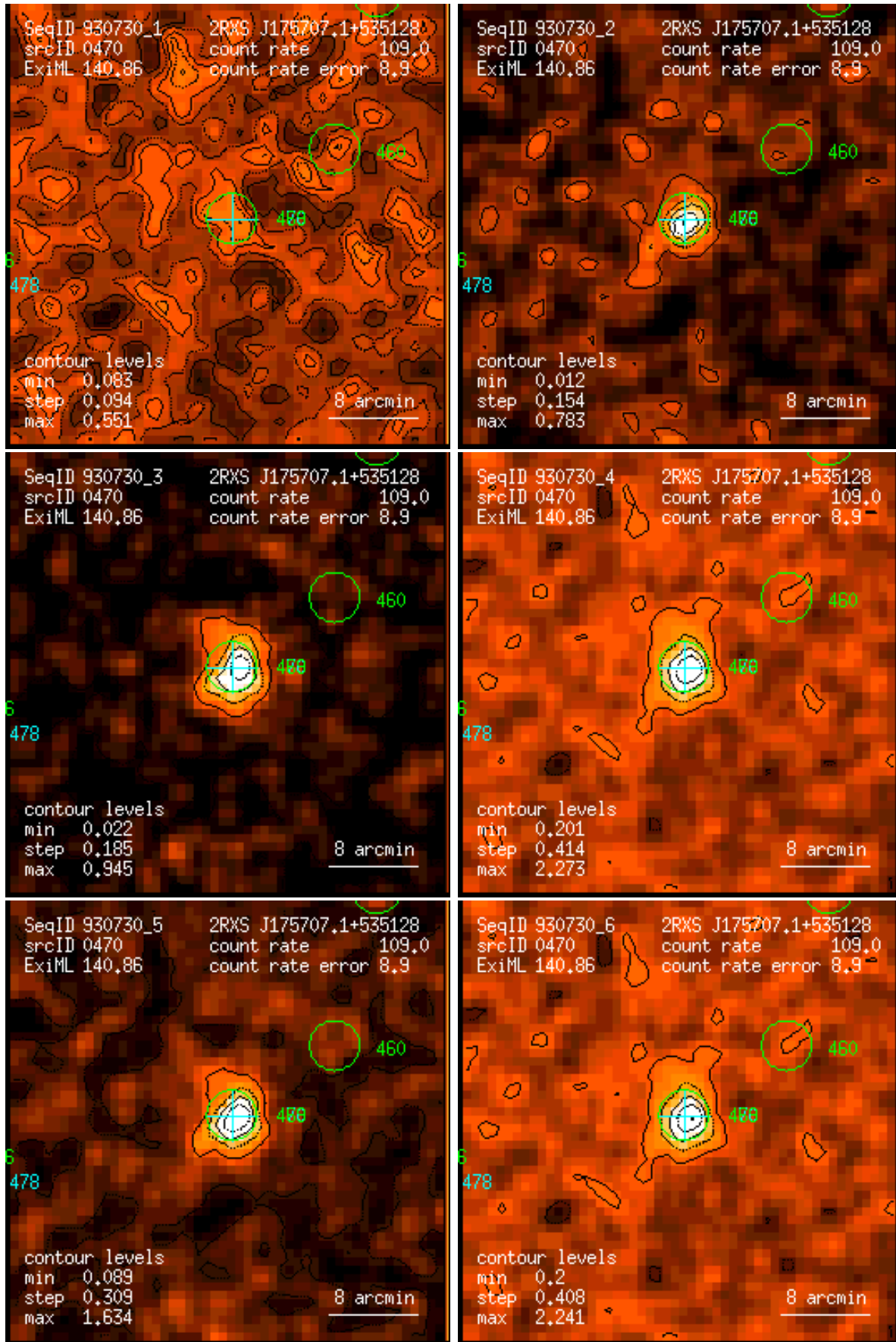
Figure 470: RASS 930730: detection 0470: band rate images, Gaussian filter: (1) PSPC channels 11 – 41, (2) 52 – 90, (3) 91 – 201, (4) 11 – 235, (5) 52 – 201, (6) 11 – 201. Broad band rates in counts/ks. Band rate contour levels in counts/ks/arcmin 2 .
